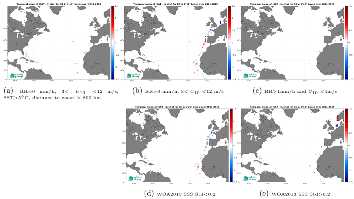
Figure 14: Temporal mean gridded over spatial boxes of size 1^\circ \times 1^\circ of \Delta\text{SSS} (Aquarius SSS L2 CAP v5 (JPL) - TSG (Polarstern)) for 5 different subdatasets corresponding to:RR=0 mm/h, 3 < U_{10} < 12 m/s, SST > 5°C, distance to coast > 800 km (a), RR=0 mm/h, 3 < U_{10} < 12 m/s (b), RR > 1mm/h and U_{10} < 4 m/s (c), WOA2013 SSS Std < 0.2 (d), WOA2013 SSS Std > 0.2 (e).
