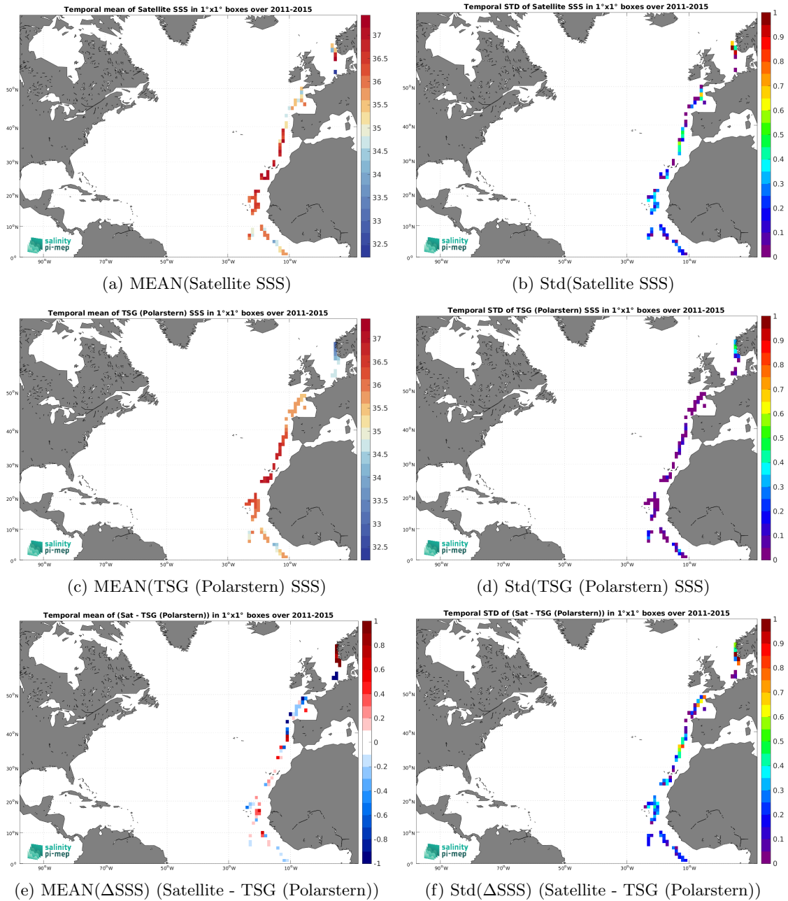
Figure 7: Temporal mean (left) and Std (right) of SSS from Aquarius SSS L2 CAP v5 (JPL) (top), TSG (Polarstern) (middle), and of \Delta SSS (Satellite - TSG (Polarstern)). Only match-up pairs are used to generate these maps.
