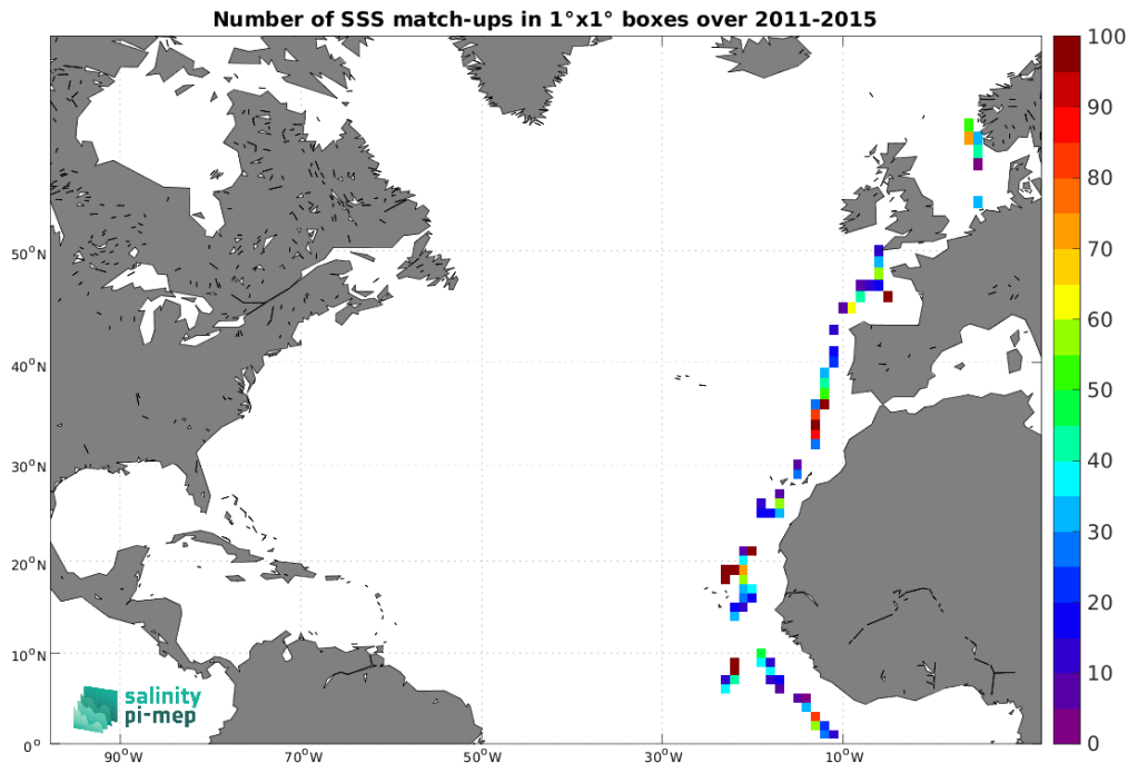
Figure 5: Number of SSS match-ups between TSG (Polarstern) SSS and the Aquarius SSS L2 CAP v5 (JPL) SSS product for the North Atlantic Ocean Pi-MEP region over 1^\circ \times 1^\circ boxes and for the full satellite product period.
