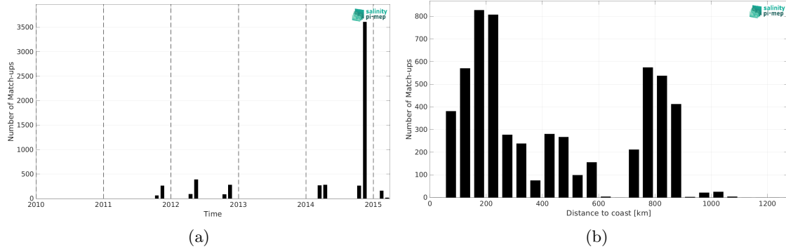
Figure 2: Number of match-ups between TSG (Polarstern) and Aquarius SSS L2 CAP v5 (JPL) SSS as a function of time (a) and as function of the distance to coast (b) over the North Atlantic Ocean Pi-MEP region and for the full satellite product period.
