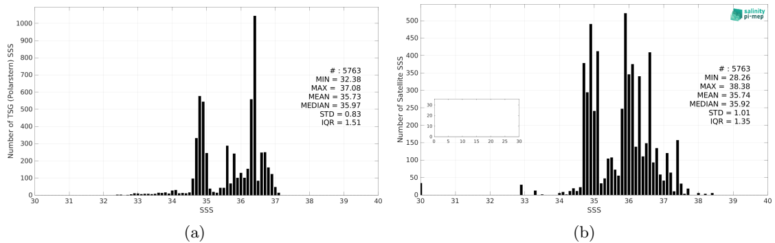
Figure 3: Histograms of SSS from TSG (Polarstern) (a) and Aquarius SSS L2 CAP v5 (JPL) (b) considering all match-up pairs per bins of 0.1 over the North Atlantic Ocean Pi-MEP region and for the full satellite product period.
