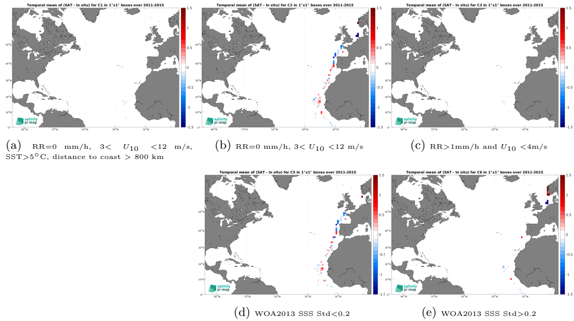
Figure 12: Temporal mean gridded over spatial boxes of size 1^\circ \times 1^\circ of \Delta\text{SSS} (Aquarius SSS L2 CAP v5 (JPL) - TSG (Polarstern)) for 5 different subdatasets corresponding to:RR=0 mm/h, 3 < U_{10} < 12 m/s, SST >5^\circ\text{C} , distance to coast > 800 km (a), RR=0 mm/h, 3 < U_{10} < 12 m/s (b), RR >1 mm/h and U_{10} < 4 m/s (c), WOA2013 SSS Std <0.2 (d), WOA2013 SSS Std >0.2 (e).
