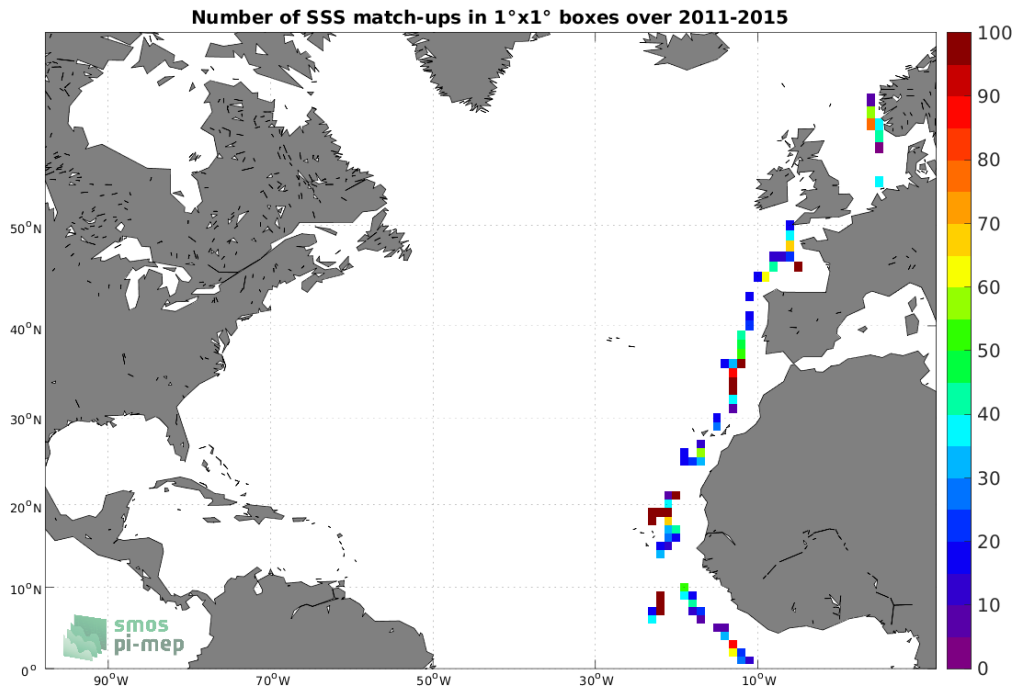
Figure 4: Number of SSS match-ups between TSG (Polarstern) SSS and the Aquarius SSS L2 CAP v5 (JPL) SSS product for the North Atlantic Ocean Pi-MEP region over 1^\circ \times 1^\circ boxes and for the full satellite product period.
