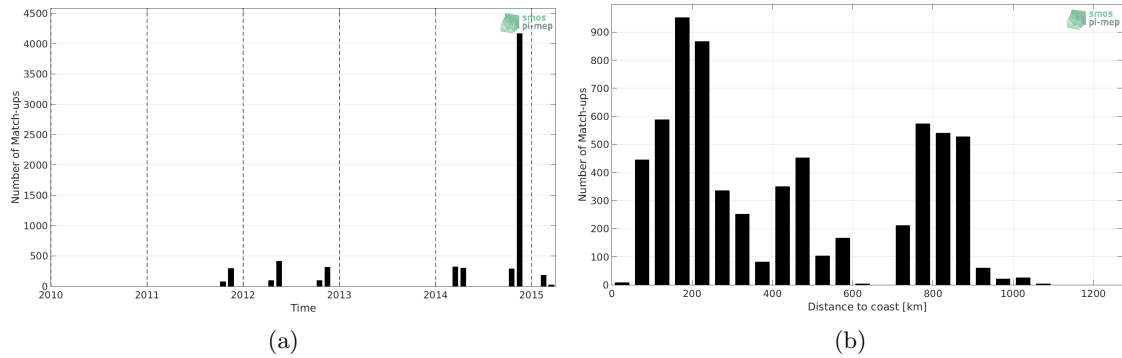
Figure 1: Number of match-ups between TSG-POLARSTERN and Aquarius-L2-JPL-V5 SSS as a function of time (a) and as function of the distance to coast (b) over the North Atlantic Ocean Pi-MEP region and for the full satellite product period.
