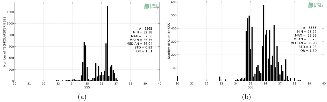
Figure 2: Histograms of SSS from TSG-POLARSTERN (a) and Aquarius-L2-JPL-V5 (b) considering all match-up pairs per bins of 0.1 over the North Atlantic Ocean Pi-MEP region and for the full satellite product period.
