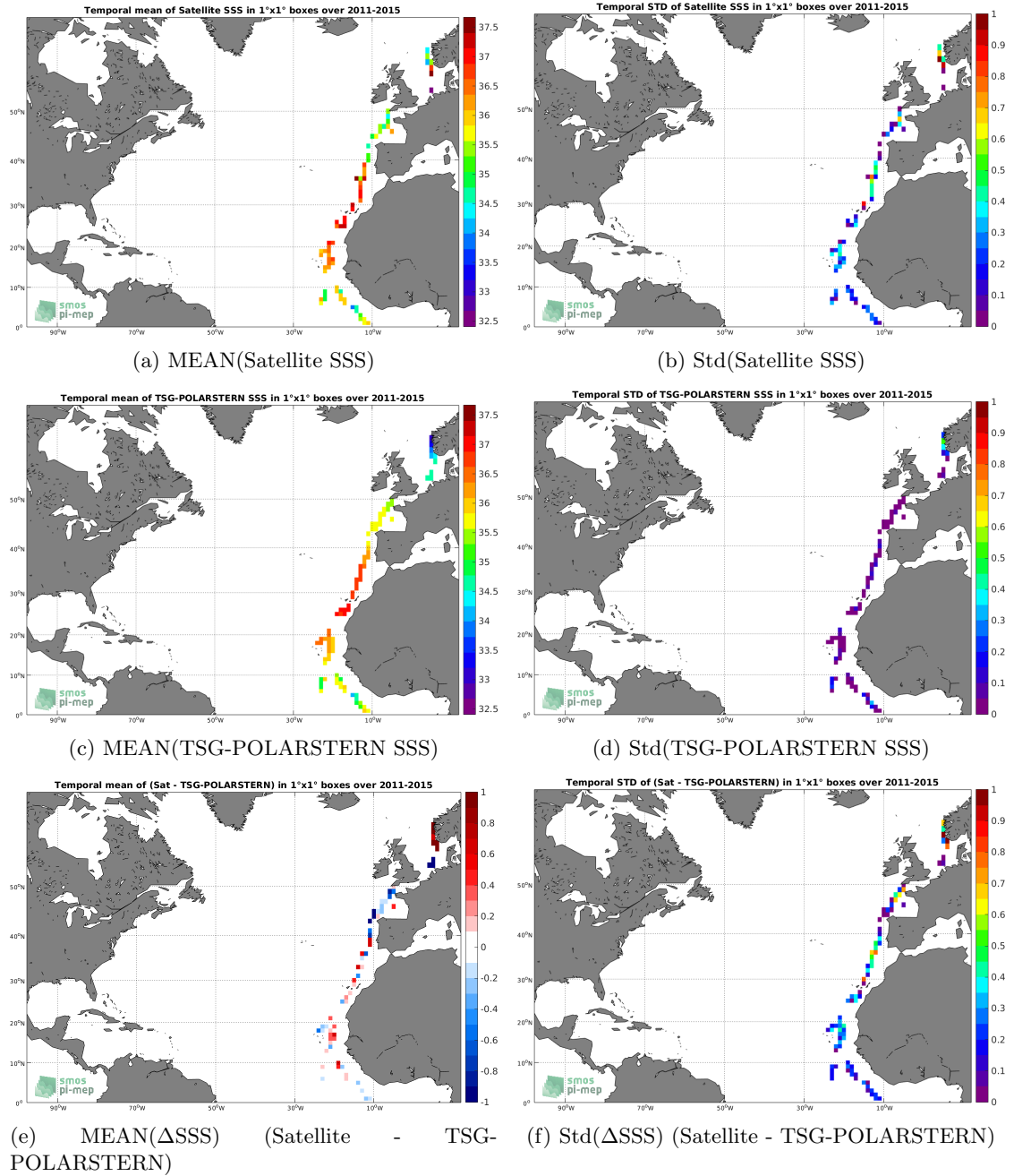
Figure 6: Temporal mean (left) and Std (right) of SSS from Aquarius-L2-JPL-V5 (top), TSG-POLARSTERN (middle), and of \Delta SSS (Satellite - TSG-POLARSTERN). Only match-up pairs are used to generate these maps.
