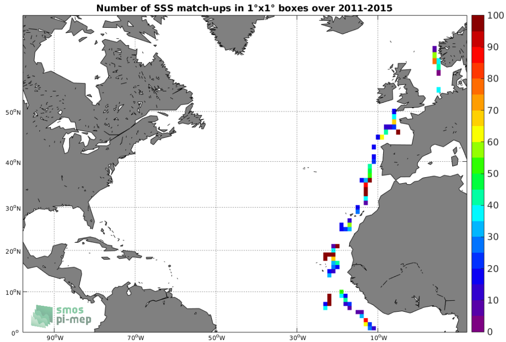
Figure 4: Number of SSS match-ups between TSG-POLARSTERN SSS and the Aquarius-L2-JPL-V5 SSS product for the North Atlantic Ocean Pi-MEP region over 1^\circ \times 1^\circ boxes and for the full satellite product period.
