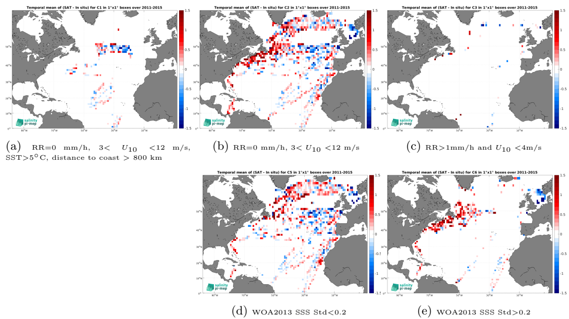
Figure 14: Temporal mean gridded over spatial boxes of size 1^\circ \times 1^\circ of \Delta\text{SSS} (Aquarius SSS L2 CAP v5 (JPL) - TSG (LEGOS-DM)) for 5 different subdatasets corresponding to:RR=0 mm/h, 3 < U_{10} < 12 m/s, SST >5^\circ\text{C} , distance to coast > 800 km (a), RR=0 mm/h, 3 < U_{10} < 12 m/s (b), RR >1 mm/h and U_{10} < 4 m/s (c), WOA2013 SSS Std <0.2 (d), WOA2013 SSS Std >0.2 (e).
