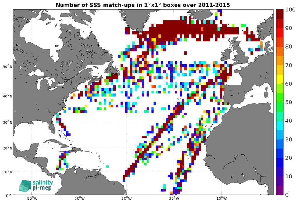
Figure 5: Number of SSS match-ups between TSG (LEGOS-DM) SSS and the Aquarius SSS L2 CAP v5 (JPL) SSS product for the North Atlantic Ocean Pi-MEP region over 1^\circ \times 1^\circ boxes and for the full satellite product period.
