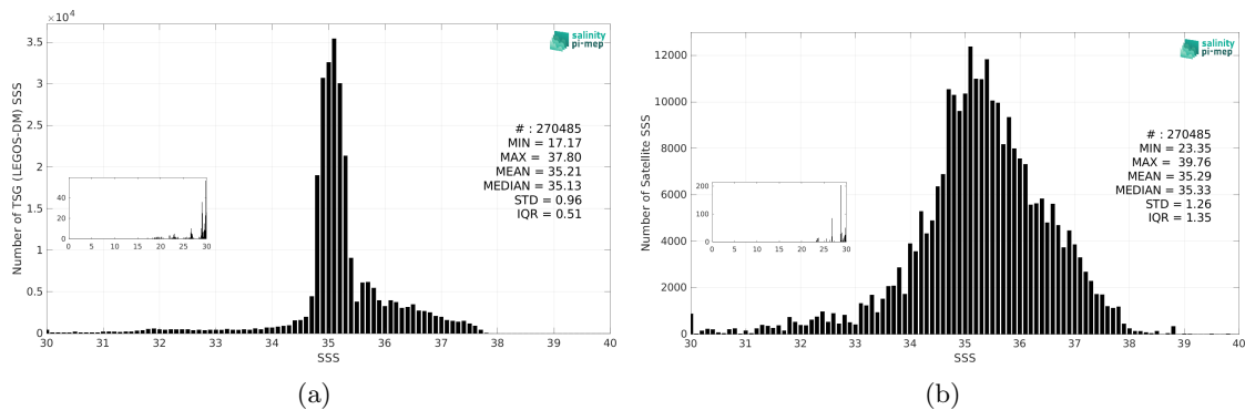
Figure 3: Histograms of SSS from TSG (LEGOS-DM) (a) and Aquarius SSS L2 CAP v5 (JPL) (b) considering all match-up pairs per bins of 0.1 over the North Atlantic Ocean Pi-MEP region and for the full satellite product period.
