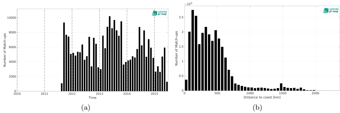
Figure 2: Number of match-ups between TSG (LEGOS-DM) and Aquarius SSS L2 CAP v5 (JPL) SSS as a function of time (a) and as function of the distance to coast (b) over the North Atlantic Ocean Pi-MEP region and for the full satellite product period.
