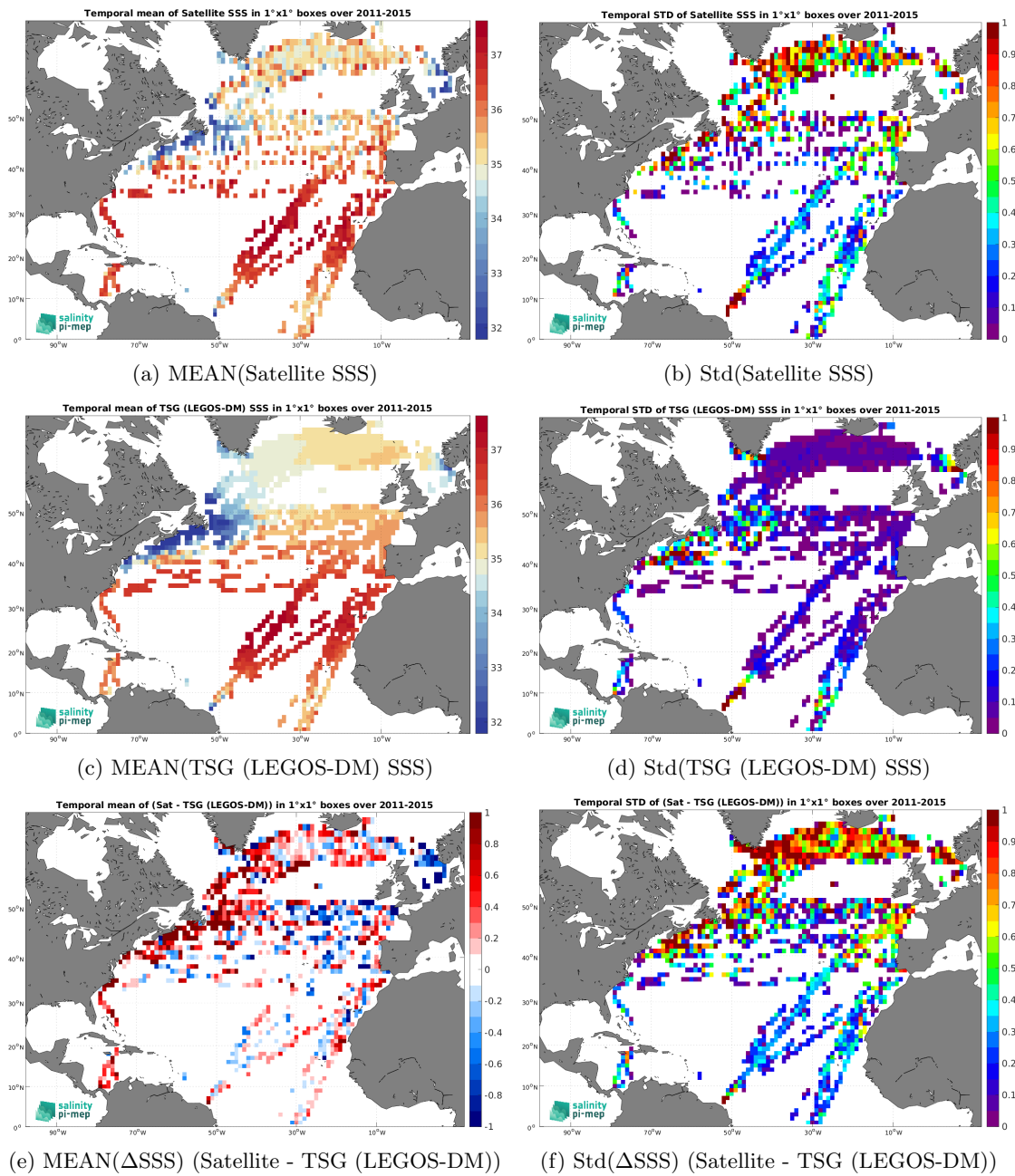
Figure 7: Temporal mean (left) and Std (right) of SSS from Aquarius SSS L2 CAP v5 (JPL) (top), TSG (LEGOS-DM) (middle), and of \Delta SSS (Satellite - TSG (LEGOS-DM)). Only match-up pairs are used to generate these maps.
