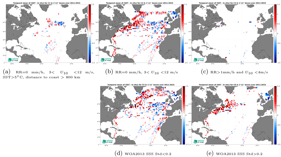
Figure 12: Temporal mean gridded over spatial boxes of size 1^\circ \times 1^\circ of \Delta\text{SSS} (Aquarius SSS L2 CAP v5 (JPL) - TSG (LEGOS-DM)) for 5 different subdatasets corresponding to:RR=0 mm/h, 3 < U_{10} < 12 m/s, SST >5^\circ\text{C} , distance to coast > 800 km (a), RR=0 mm/h, 3 < U_{10} < 12 m/s (b), RR >1 mm/h and U_{10} < 4 m/s (c), WOA2013 SSS Std <0.2 (d), WOA2013 SSS Std >0.2 (e).
