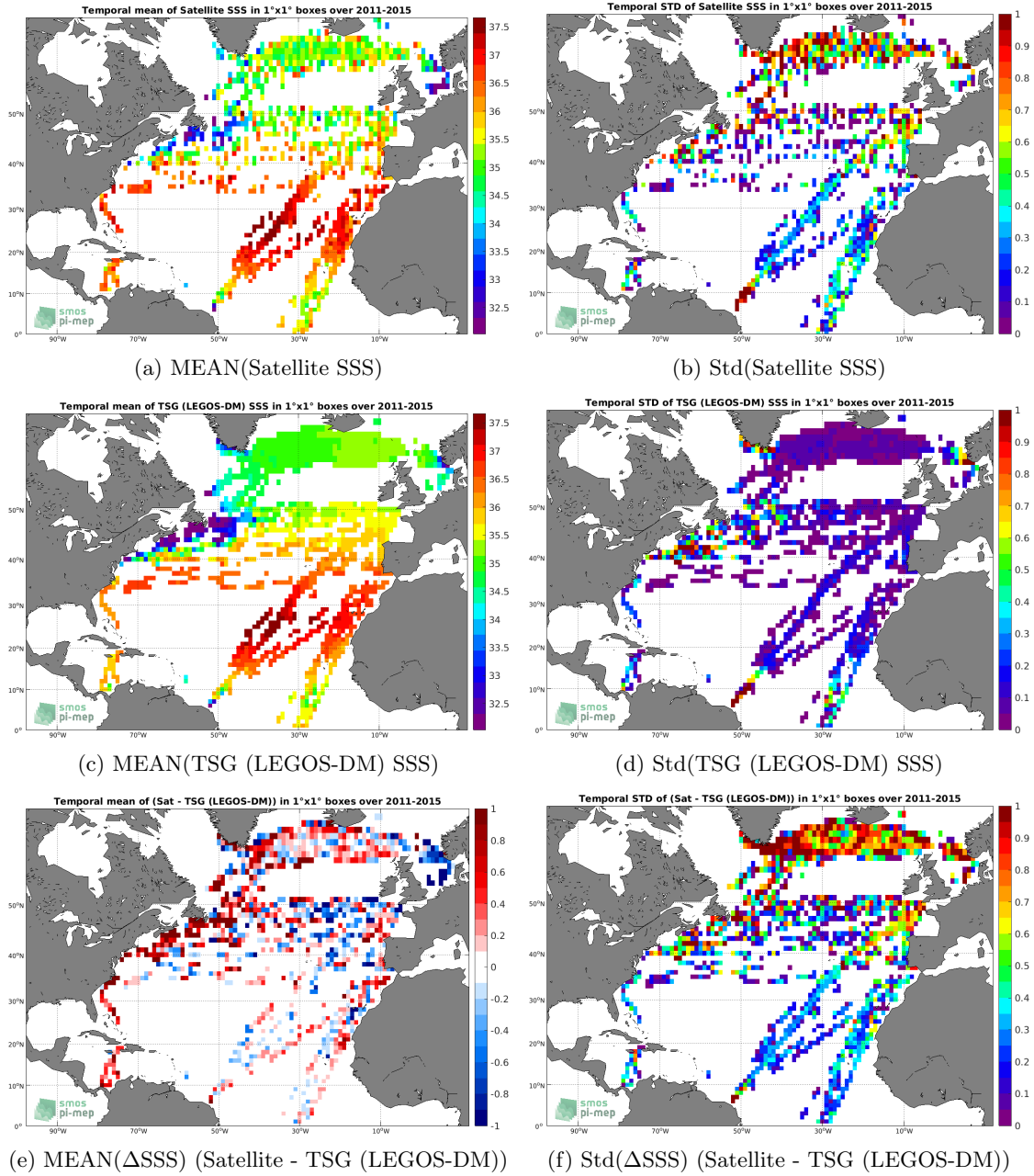
Figure 6: Temporal mean (left) and Std (right) of SSS from Aquarius SSS L2 CAP v5 (JPL) (top), TSG (LEGOS-DM) (middle), and of \Delta SSS (Satellite - TSG (LEGOS-DM)). Only match-up pairs are used to generate these maps.
