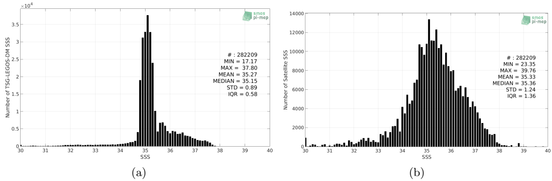
Figure 2: Histograms of SSS from TSG-LEGOS-DM (a) and Aquarius-L2-JPL-V5 (b) considering all match-up pairs per bins of 0.1 over the North Atlantic Ocean Pi-MEP region and for the full satellite product period.
