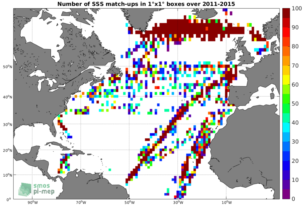
Figure 4: Number of SSS match-ups between TSG-LEGOS-DM SSS and the Aquarius-L2-JPL-V5 SSS product for the North Atlantic Ocean Pi-MEP region over 1^\circ \times 1^\circ boxes and for the full satellite product period.
