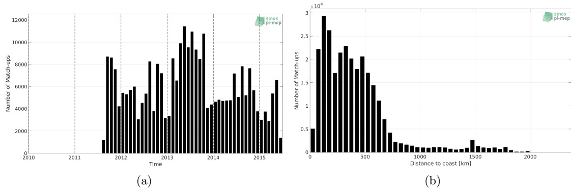
Figure 1: Number of match-ups between TSG-LEGOS-DM and Aquarius-L2-JPL-V5 SSS as a function of time (a) and as function of the distance to coast (b) over the North Atlantic Ocean Pi-MEP region and for the full satellite product period.
