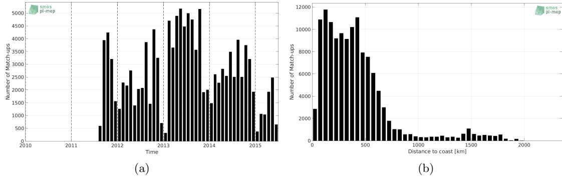
Figure 1: Number of match-ups between TSG-LEGOS-DM and Aquarius-L2-JPL-V5 SSS as a function of time (a) and as function of the distance to coast (b) over the North Atlantic Ocean Pi-MEP region and for the full satellite product period.
