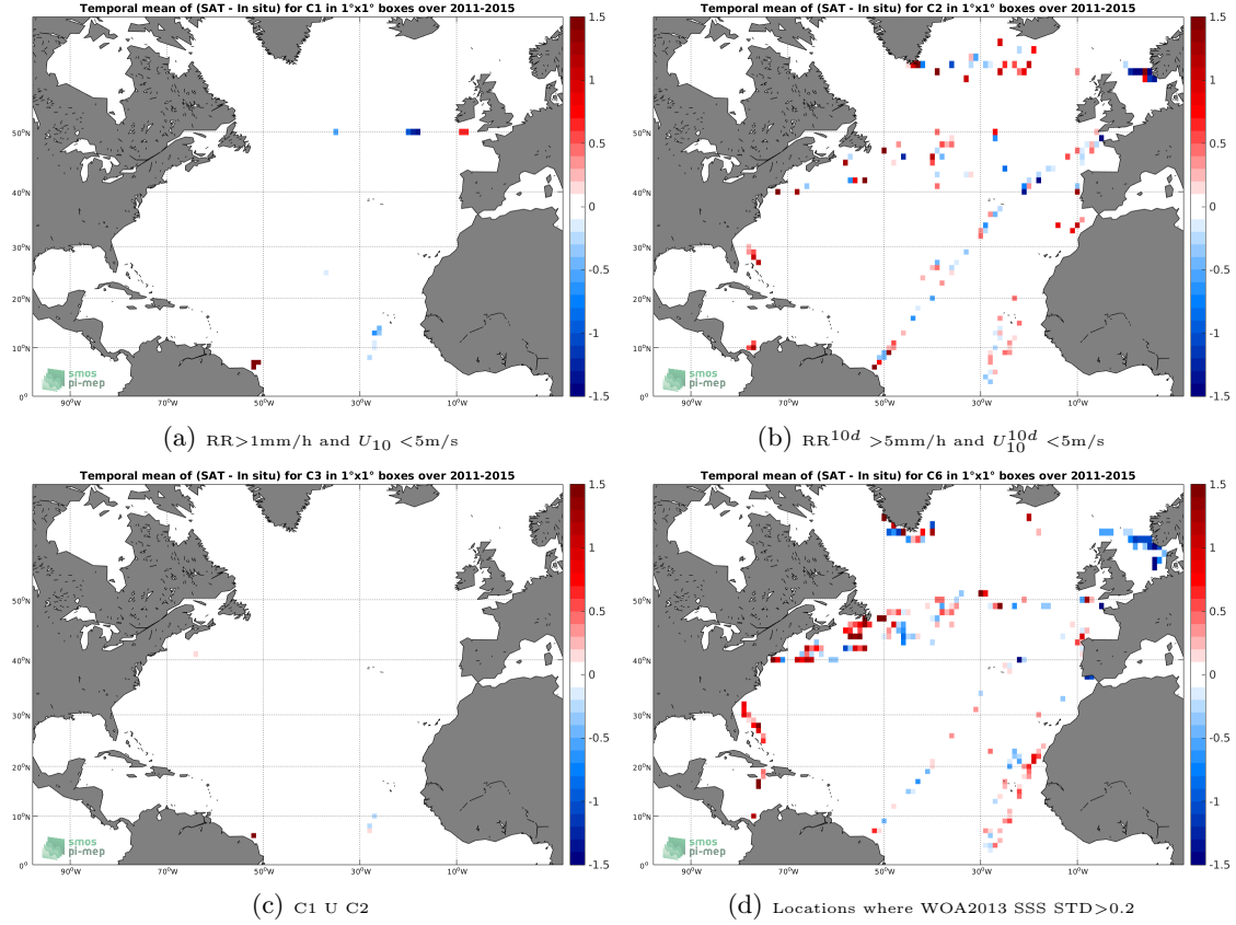
Figure 12: Temporal mean gridded over spatial boxes of size 1^\circ \times 1^\circ of \Delta SSS (Aquarius-L2-JPL-V5 - TSG-LEGOS-DM) for 4 different subdatasets corresponding to: RR > 1\text{mm/h} and U_{10} < 5\text{m/s} (a), RR^{10d} > 5\text{mm/h} and U_{10}^{10d} < 5\text{m/s} (b), C1 U C2 (c), Locations where WOA2013 SSS STD > 0.2 (d).
