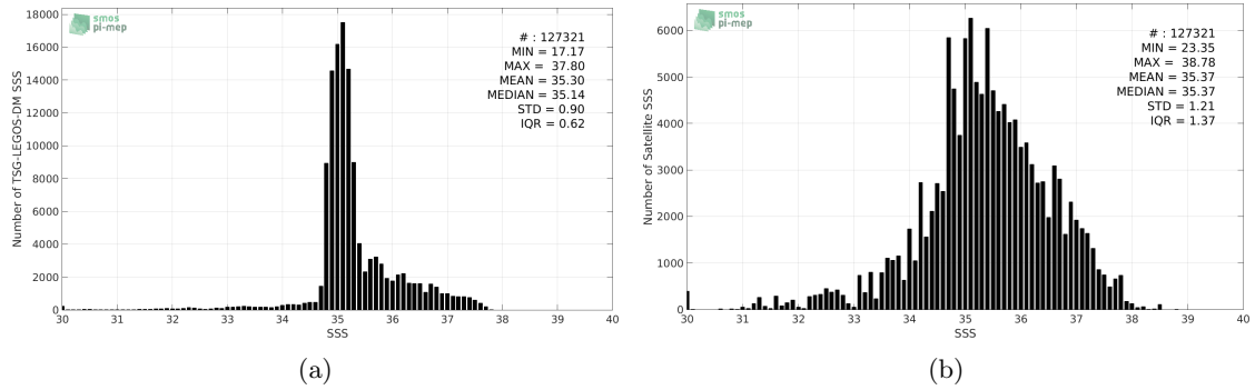
Figure 2: Histograms of SSS from TSG-LEGOS-DM (a) and Aquarius-L2-JPL-V5 (b) considering all match-up pairs per bins of 0.1 over the North Atlantic Ocean Pi-MEP region and for the full satellite product period.
