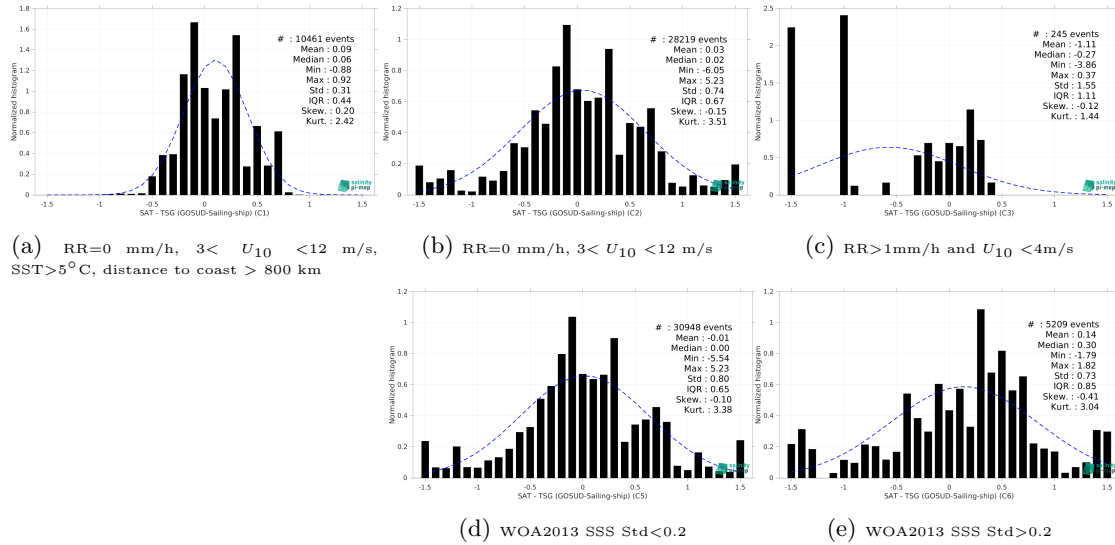
Figure 15: Normalized histogram of \Delta\text{SSS} (Aquarius SSS L2 CAP v5 (JPL) - TSG (GOSUD-Sailing-ship)) for 5 different subdatasets corresponding to: RR=0 mm/h, 3 < U_{10} < 12 m/s, SST>5°C, distance to coast > 800 km (a), RR=0 mm/h, 3 < U_{10} < 12 m/s (b), RR>1mm/h and U_{10} < 4 m/s (c), WOA2013 SSS Std<0.2 (d), WOA2013 SSS Std>0.2 (e).
