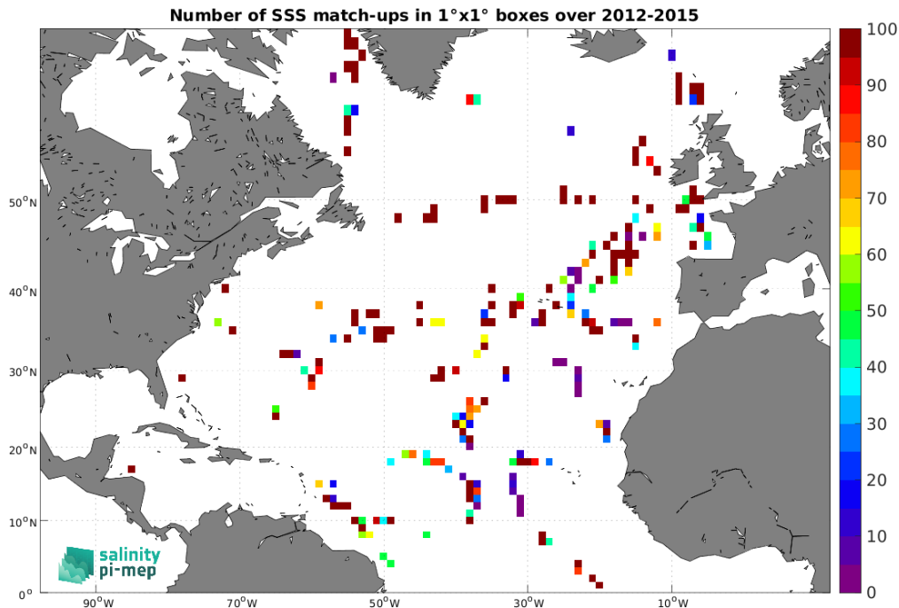
Figure 5: Number of SSS match-ups between TSG (GOSUD-Sailing-ship) SSS and the Aquarius SSS L2 CAP v5 (JPL) SSS product for the North Atlantic Ocean Pi-MEP region over 1^\circ \times 1^\circ boxes and for the full satellite product period.
