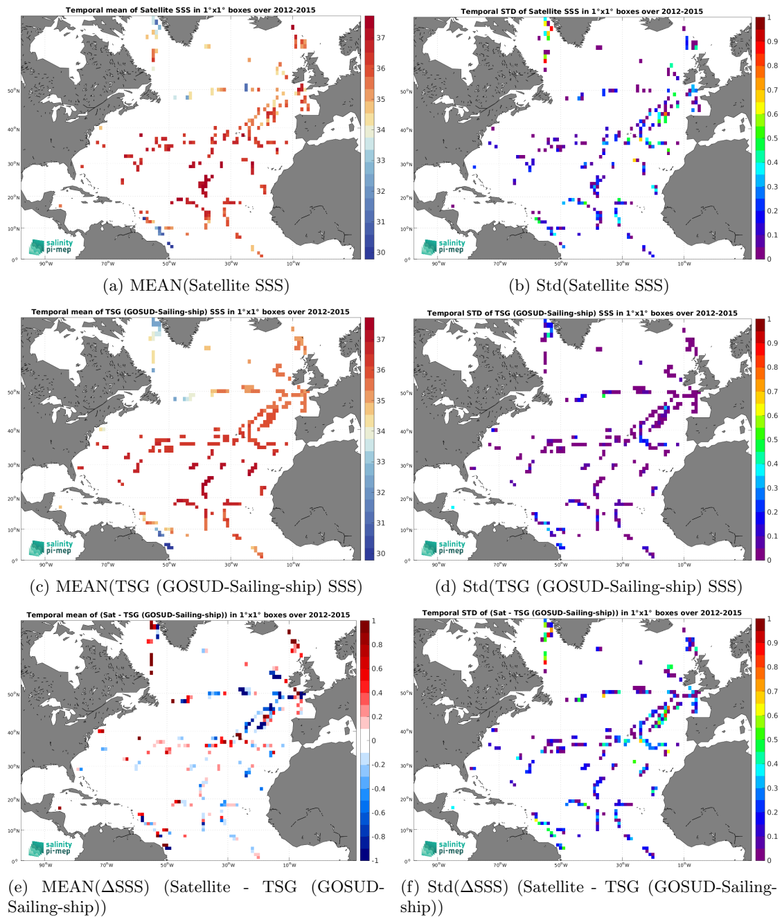
Figure 7: Temporal mean (left) and Std (right) of SSS from Aquarius SSS L2 CAP v5 (JPL) (top), TSG (GOSUD-Sailing-ship) (middle), and of \Delta SSS (Satellite - TSG (GOSUD-Sailing-ship)). Only match-up pairs are used to generate these maps.
