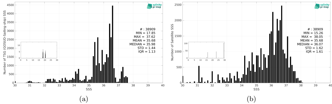
Figure 3: Histograms of SSS from TSG (GOSUD-Sailing-ship) (a) and Aquarius SSS L2 CAP v5 (JPL) (b) considering all match-up pairs per bins of 0.1 over the North Atlantic Ocean Pi-MEP region and for the full satellite product period.
