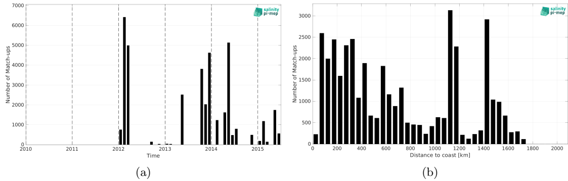
Figure 2: Number of match-ups between TSG (GOSUD-Sailing-ship) and Aquarius SSS L2 CAP v5 (JPL) SSS as a function of time (a) and as function of the distance to coast (b) over the North Atlantic Ocean Pi-MEP region and for the full satellite product period.
