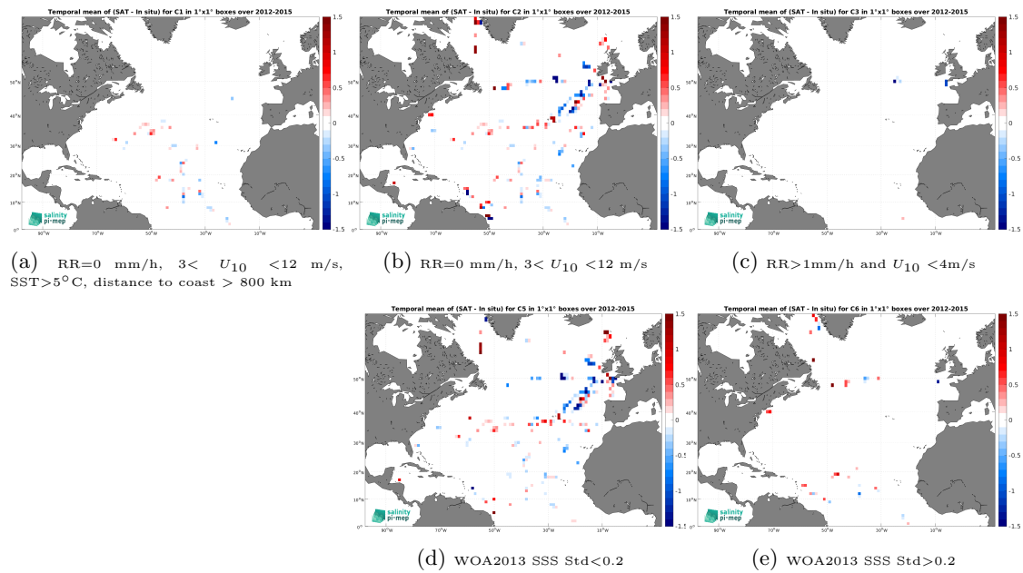
Figure 14: Temporal mean gridded over spatial boxes of size 1^\circ \times 1^\circ of \Delta\text{SSS} (Aquarius SSS L2 CAP v5 (JPL) - TSG (GOSUD-Sailing-ship)) for 5 different subdatasets corresponding to:RR=0 mm/h, 3 < U_{10} < 12 m/s, SST > 5°C, distance to coast > 800 km (a), RR=0 mm/h, 3 < U_{10} < 12 m/s (b), RR > 1mm/h and U_{10} < 4 m/s (c), WOA2013 SSS Std < 0.2 (d), WOA2013 SSS Std > 0.2 (e).
