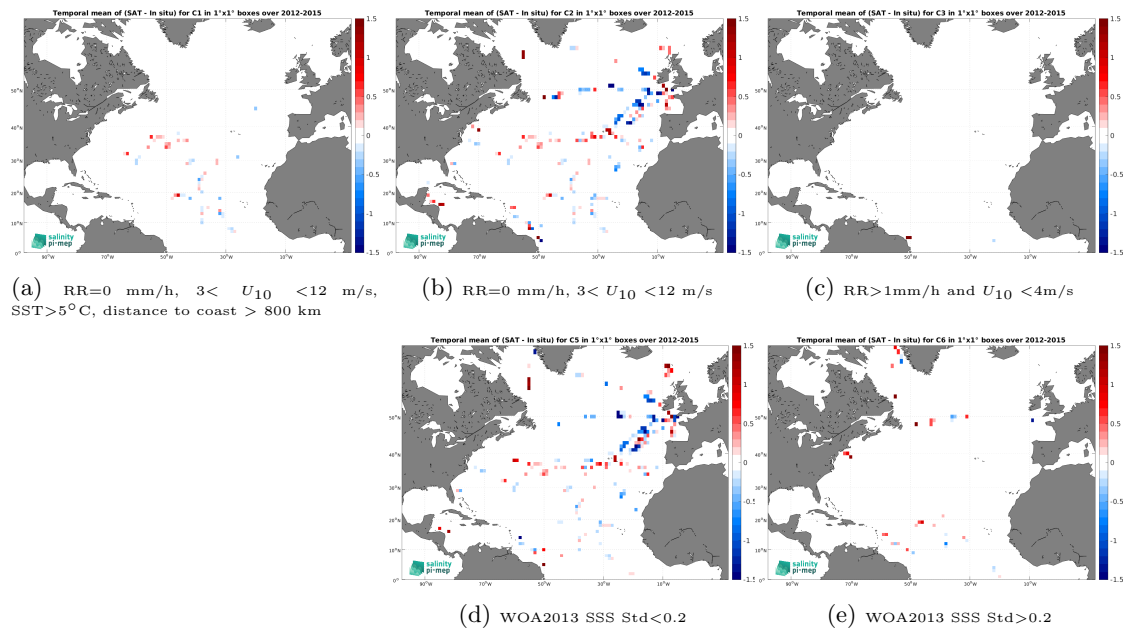
Figure 12: Temporal mean gridded over spatial boxes of size 1^\circ \times 1^\circ of \Delta\text{SSS} (Aquarius SSS L2 CAP v5 (JPL) - TSG (GOSUD-Sailing-ship)) for 5 different subdatasets corresponding to:RR=0 mm/h, 3 < U_{10} < 12 m/s, SST >5^\circ\text{C} , distance to coast > 800 km (a), RR=0 mm/h, 3 < U_{10} < 12 m/s (b), RR >1 mm/h and U_{10} < 4 m/s (c), WOA2013 SSS Std <0.2 (d), WOA2013 SSS Std >0.2 (e).
