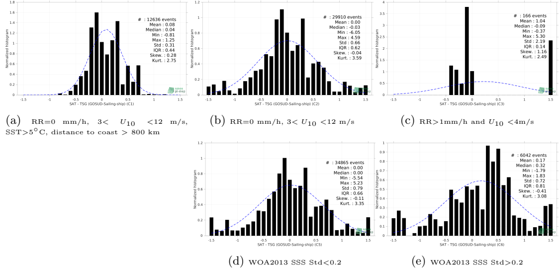
Figure 13: Normalized histogram of \Delta\text{SSS} (Aquarius SSS L2 CAP v5 (JPL) - TSG (GOSUD-Sailing-ship)) for 5 different subdatasets corresponding to: RR=0 mm/h, 3 < U_{10} < 12 m/s, SST>5°C, distance to coast > 800 km (a), RR=0 mm/h, 3 < U_{10} < 12 m/s (b), RR>1mm/h and U_{10} < 4 m/s (c), WOA2013 SSS Std<0.2 (d), WOA2013 SSS Std>0.2 (e).
