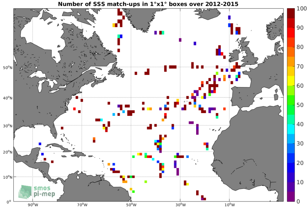
Figure 4: Number of SSS match-ups between TSG-GOSUD-Sailing-ship SSS and the Aquarius-L2-JPL-V5 SSS product for the North Atlantic Ocean Pi-MEP region over 1^\circ \times 1^\circ boxes and for the full satellite product period.
