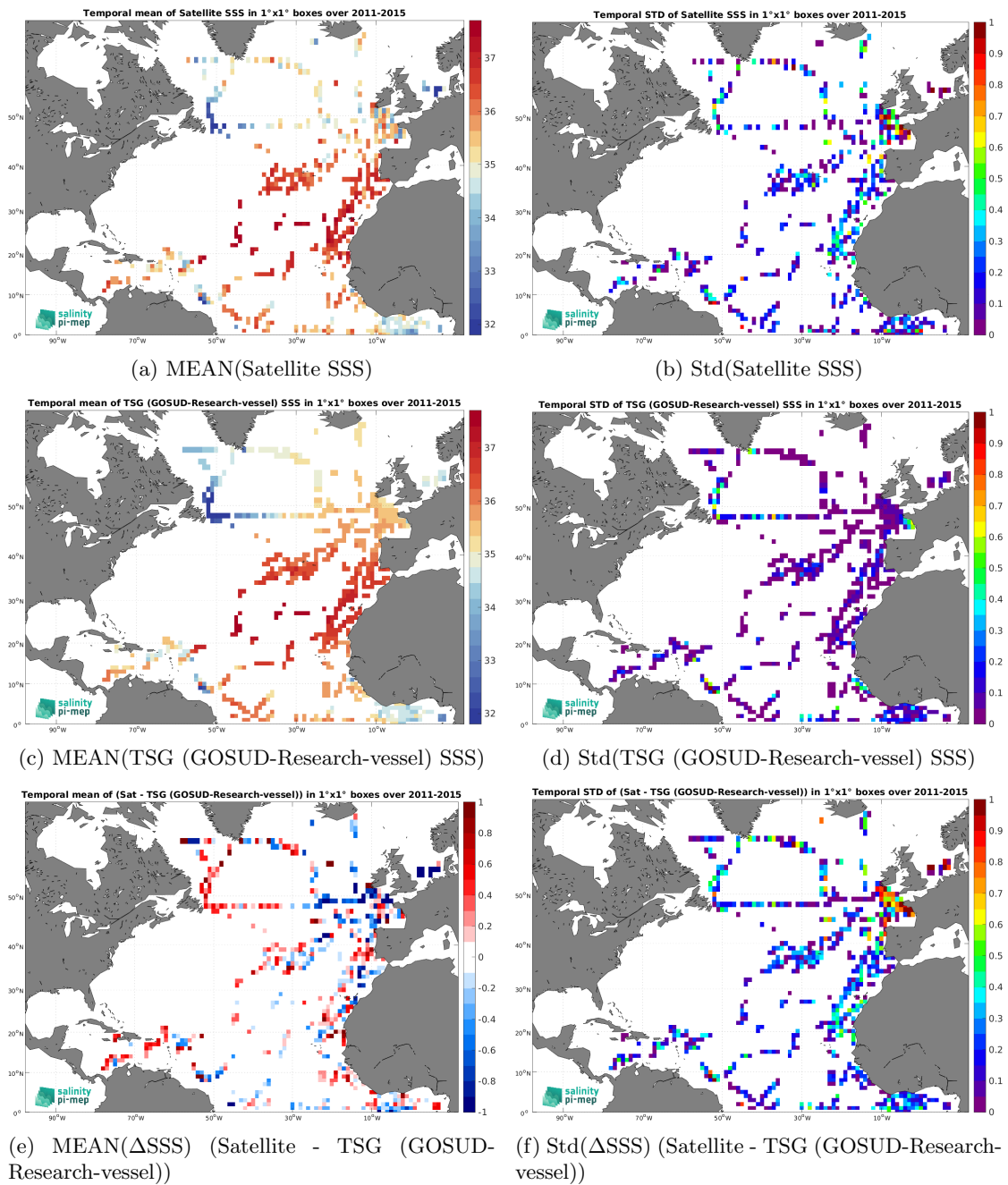
Figure 7: Temporal mean (left) and Std (right) of SSS from Aquarius SSS L2 CAP v5 (JPL) (top), TSG (GOSUD-Research-vessel) (middle), and of \Delta SSS (Satellite - TSG (GOSUD-Research-vessel)). Only match-up pairs are used to generate these maps.
