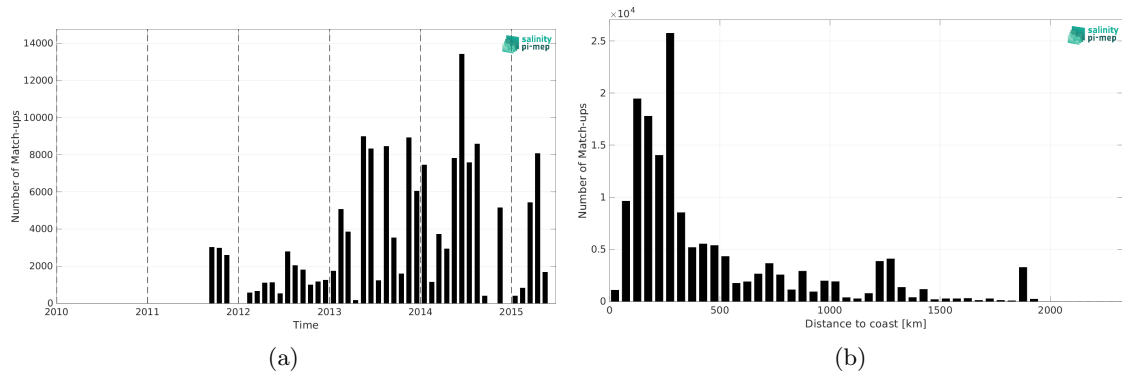
Figure 2: Number of match-ups between TSG (GOSUD-Research-vessel) and Aquarius SSS L2 CAP v5 (JPL) SSS as a function of time (a) and as function of the distance to coast (b) over the North Atlantic Ocean Pi-MEP region and for the full satellite product period.
