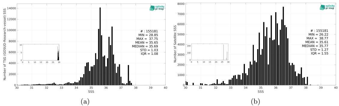
Figure 3: Histograms of SSS from TSG (GOSUD-Research-vessel) (a) and Aquarius SSS L2 CAP v5 (JPL) (b) considering all match-up pairs per bins of 0.1 over the North Atlantic Ocean Pi-MEP region and for the full satellite product period.
