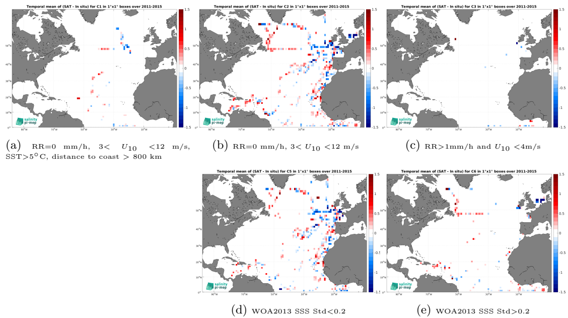
Figure 14: Temporal mean gridded over spatial boxes of size 1^\circ \times 1^\circ of \Delta SSS (Aquarius SSS L2 CAP v5 (JPL) - TSG (GOSUD-Research-vessel)) for 5 different subdatasets corresponding to:RR=0 mm/h, 3 < U_{10} < 12 m/s, SST >5^\circ\text{C} , distance to coast > 800 km (a), RR=0 mm/h, 3 < U_{10} < 12 m/s (b), RR >1 mm/h and U_{10} < 4 m/s (c), WOA2013 SSS Std <0.2 (d), WOA2013 SSS Std >0.2 (e).
