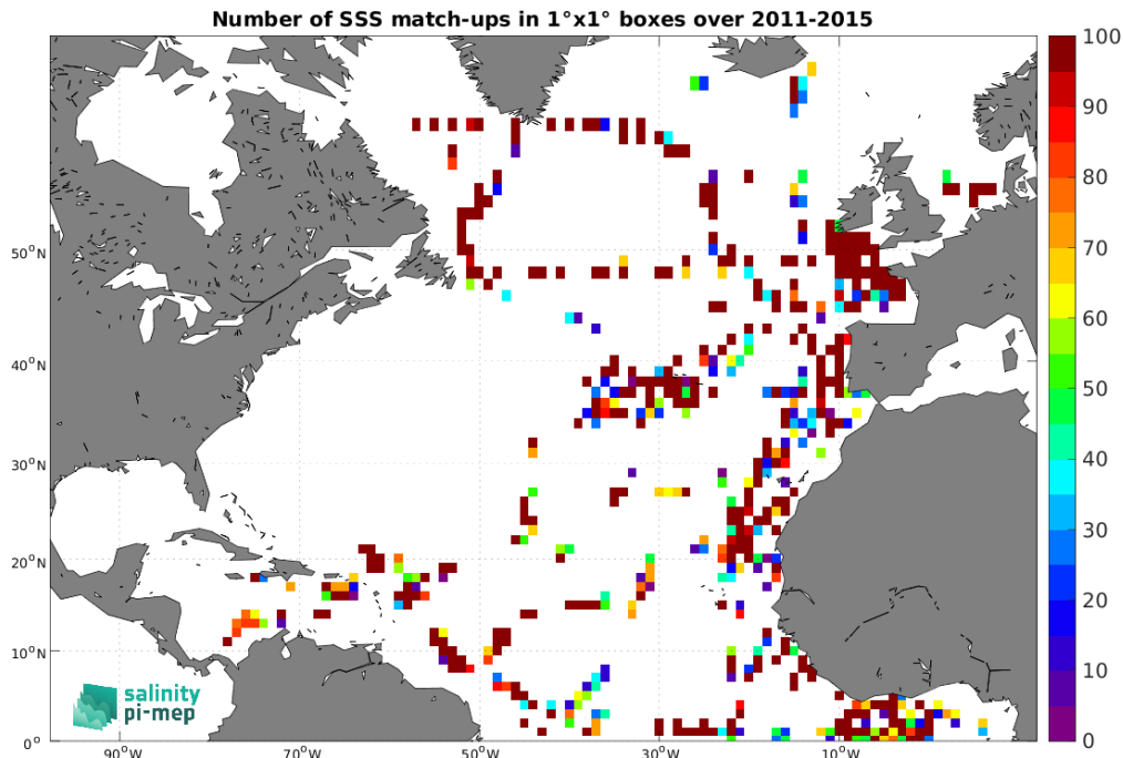
Figure 5: Number of SSS match-ups between TSG (GOSUD-Research-vessel) SSS and the Aquarius SSS L2 CAP v5 (JPL) SSS product for the North Atlantic Ocean Pi-MEP region over 1^\circ \times 1^\circ boxes and for the full satellite product period.
