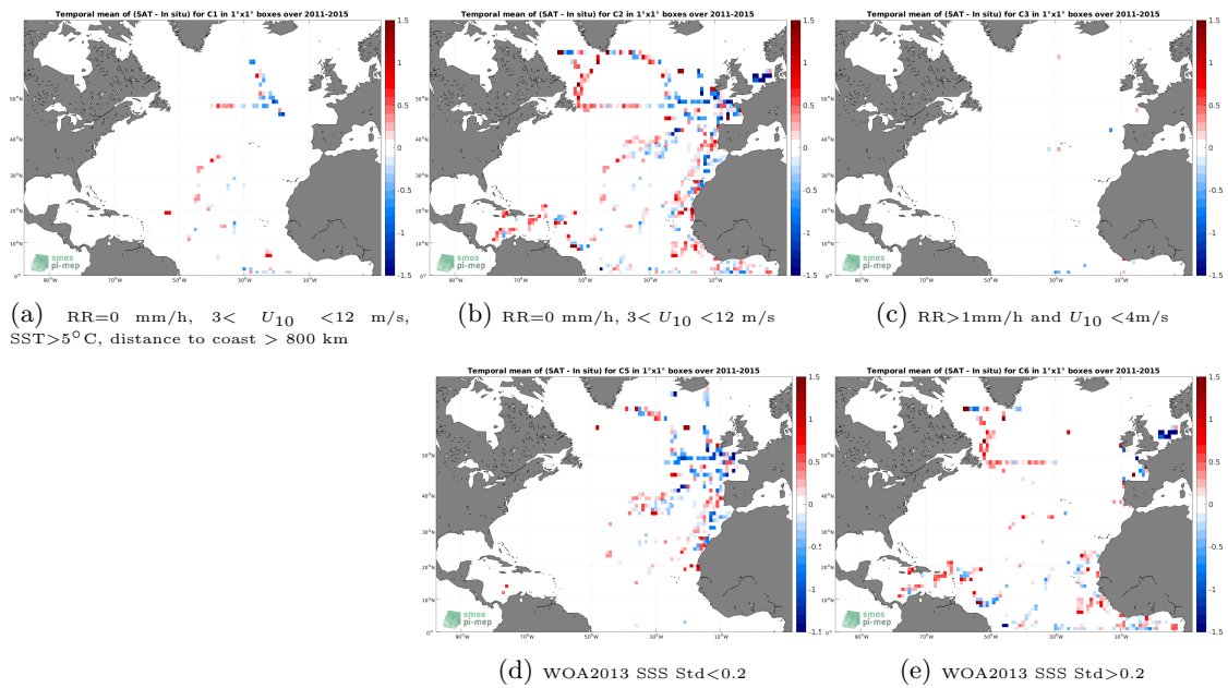
Figure 12: Temporal mean gridded over spatial boxes of size 1^\circ \times 1^\circ of \Delta\text{SSS} (Aquarius SSS L2 CAP v5 (JPL) - TSG (GOSUD-Research-vessel)) for 5 different subdatasets corresponding to:RR=0 mm/h, 3 < U_{10} < 12 m/s, SST > 5°C, distance to coast > 800 km (a), RR=0 mm/h, 3 < U_{10} < 12 m/s (b), RR > 1mm/h and U_{10} < 4 m/s (c), WOA2013 SSS Std < 0.2 (d), WOA2013 SSS Std > 0.2 (e).
