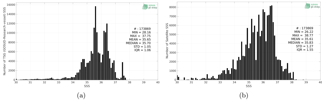
Figure 2: Histograms of SSS from TSG (GOSUD-Research-vessel) (a) and Aquarius SSS L2 CAP v5 (JPL) (b) considering all match-up pairs per bins of 0.1 over the North Atlantic Ocean Pi-MEP region and for the full satellite product period.
