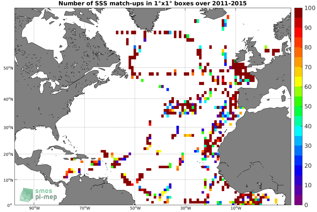
Figure 4: Number of SSS match-ups between TSG (GOSUD-Research-vessel) SSS and the Aquarius SSS L2 CAP v5 (JPL) SSS product for the North Atlantic Ocean Pi-MEP region over 1^\circ \times 1^\circ boxes and for the full satellite product period.
