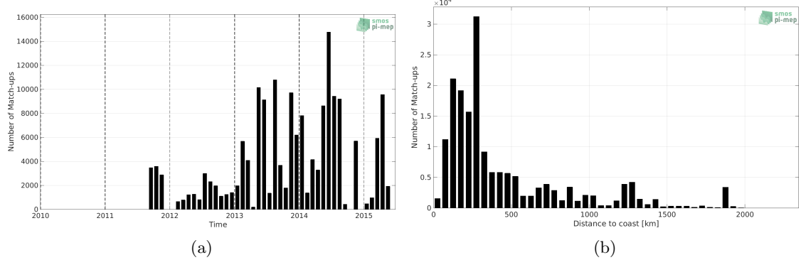
Figure 1: Number of match-ups between TSG (GOSUD-Research-vessel) and Aquarius SSS L2 CAP v5 (JPL) SSS as a function of time (a) and as function of the distance to coast (b) over the North Atlantic Ocean Pi-MEP region and for the full satellite product period.
