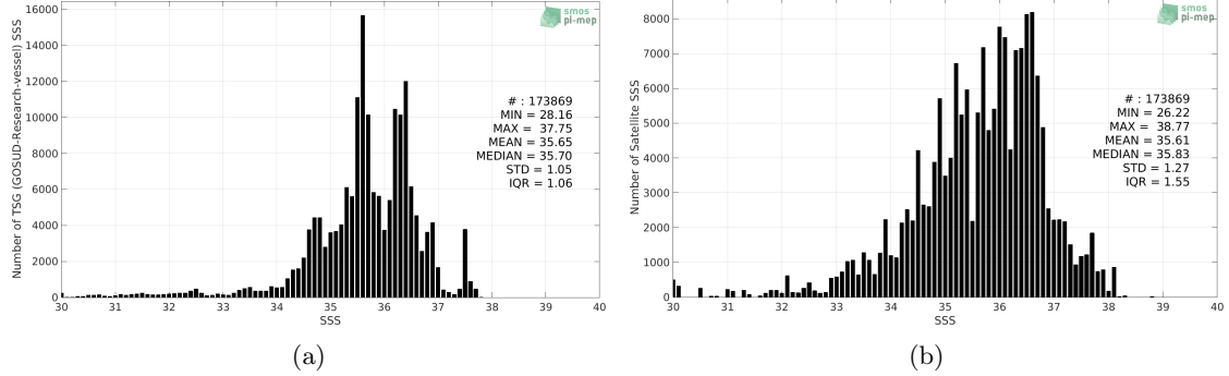
Figure 2: Histograms of SSS from TSG (GOSUD-Research-vessel) (a) and Aquarius SSS L2 CAP v5 (JPL) (b) considering all match-up pairs per bins of 0.1 over the North Atlantic Ocean Pi-MEP region and for the full satellite product period.
