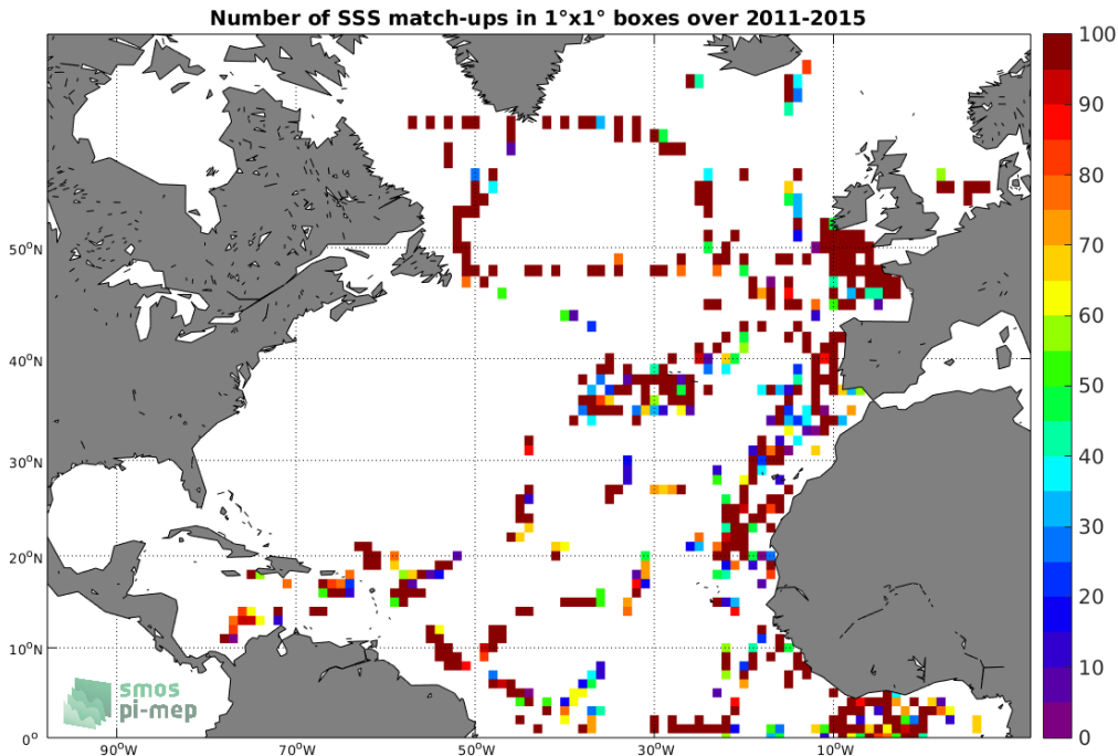
Figure 4: Number of SSS match-ups between TSG-GOSUD-Research-vessel SSS and the Aquarius-L2-JPL-V5 SSS product for the North Atlantic Ocean Pi-MEP region over 1^{\circ} \times 1^{\circ} boxes and for the full satellite product period.
