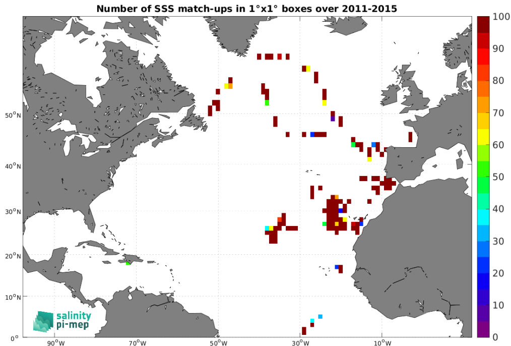
Figure 5: Number of SSS match-ups between TSG (CSIC-UTM) SSS and the Aquarius SSS L2 CAP v5 (JPL) SSS product for the North Atlantic Ocean Pi-MEP region over 1^\circ \times 1^\circ boxes and for the full satellite product period.
