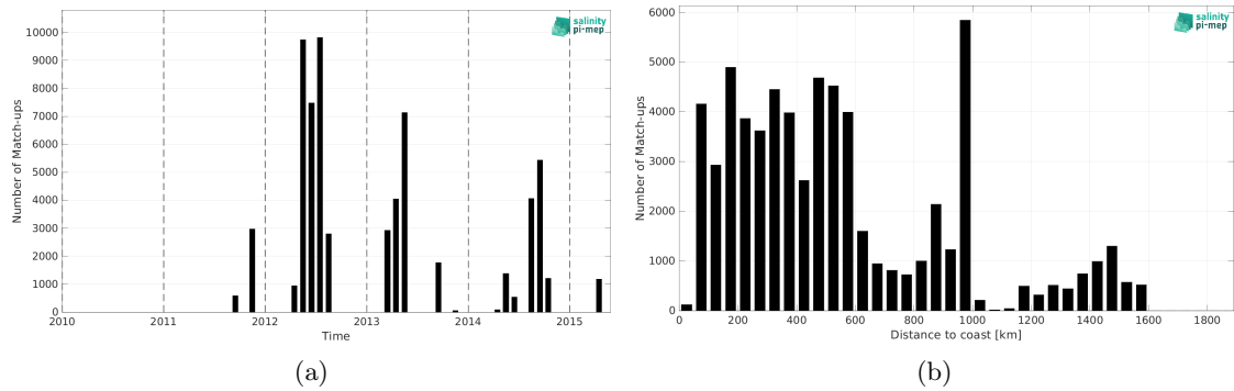
Figure 2: Number of match-ups between TSG (CSIC-UTM) and Aquarius SSS L2 CAP v5 (JPL) SSS as a function of time (a) and as function of the distance to coast (b) over the North Atlantic Ocean Pi-MEP region and for the full satellite product period.
