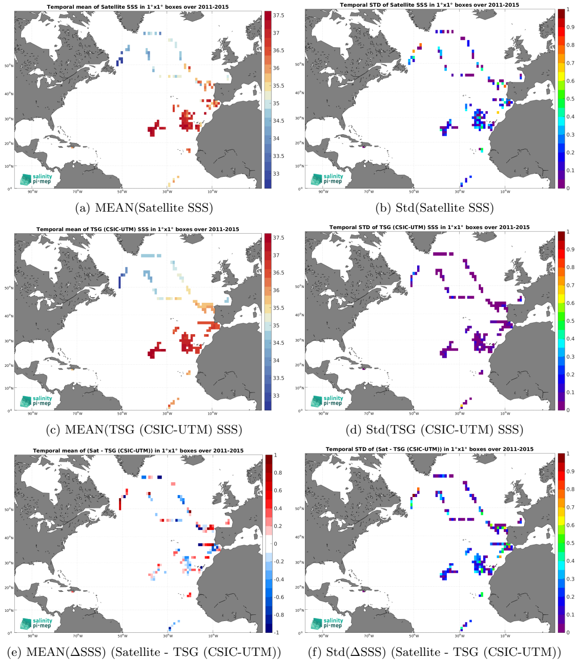
Figure 7: Temporal mean (left) and Std (right) of SSS from Aquarius SSS L2 CAP v5 (JPL) (top), TSG (CSIC-UTM) (middle), and of \Delta SSS (Satellite - TSG (CSIC-UTM)). Only match-up pairs are used to generate these maps.
