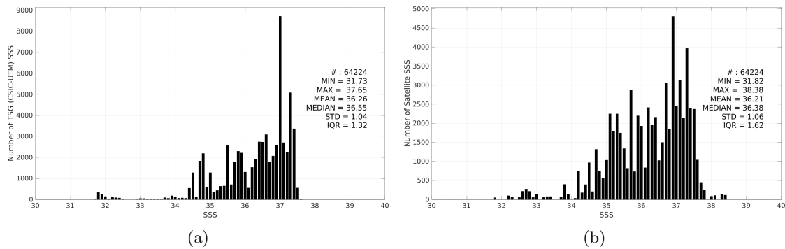
Figure 3: Histograms of SSS from TSG (CSIC-UTM) (a) and Aquarius SSS L2 CAP v5 (JPL) (b) considering all match-up pairs per bins of 0.1 over the North Atlantic Ocean Pi-MEP region and for the full satellite product period.
