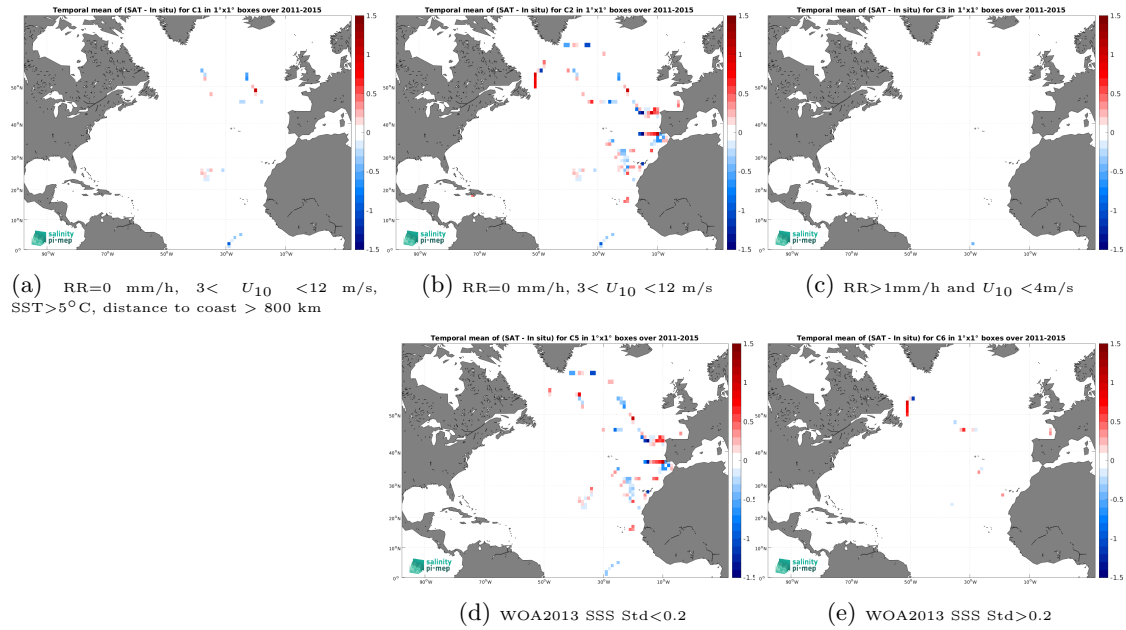
Figure 12: Temporal mean gridded over spatial boxes of size 1^\circ \times 1^\circ of \Delta\text{SSS} (Aquarius SSS L2 CAP v5 (JPL) - TSG (CSIC-UTM)) for 5 different subdatasets corresponding to:RR=0 mm/h, 3 < U_{10} < 12 m/s, SST >5^\circ\text{C} , distance to coast > 800 km (a), RR=0 mm/h, 3 < U_{10} < 12 m/s (b), RR >1 mm/h and U_{10} < 4 m/s (c), WOA2013 SSS Std <0.2 (d), WOA2013 SSS Std >0.2 (e).
