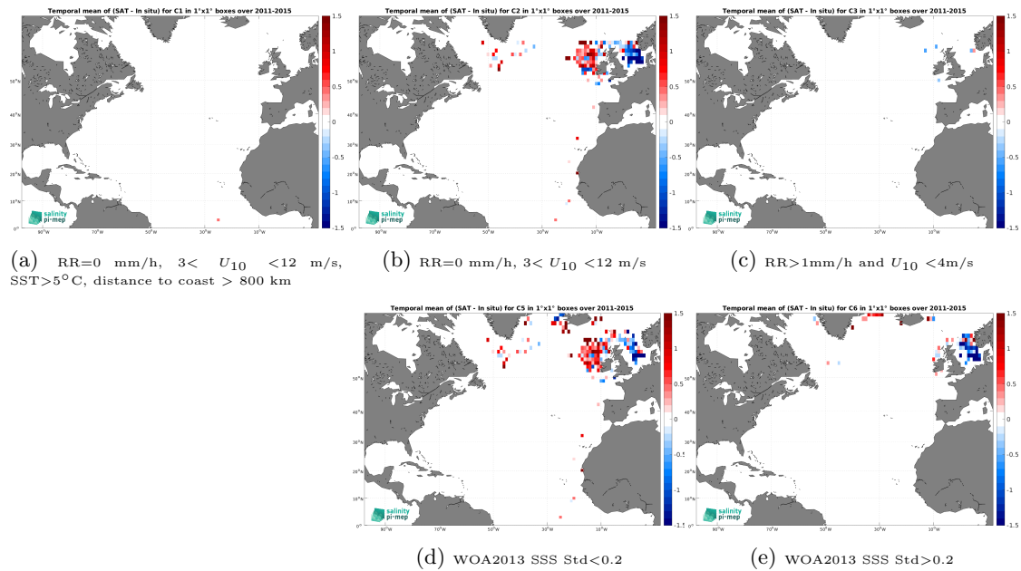
Figure 12: Temporal mean gridded over spatial boxes of size 1^\circ \times 1^\circ of \Delta\text{SSS} (Aquarius SSS L2 CAP v5 (JPL) - ICES) for 5 different subdatasets corresponding to:RR=0 mm/h, 3 < U_{10} < 12 m/s, SST >5^\circ\text{C} , distance to coast > 800 km (a), RR=0 mm/h, 3 < U_{10} < 12 m/s (b), RR >1 mm/h and U_{10} < 4 m/s (c), WOA2013 SSS Std <0.2 (d), WOA2013 SSS Std >0.2 (e).
