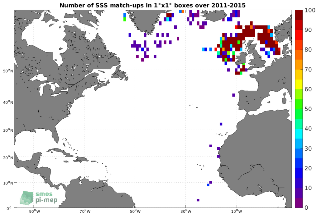
Figure 4: Number of SSS match-ups between ICES SSS and the Aquarius SSS L2 CAP v5 (JPL) SSS product for the North Atlantic Ocean Pi-MEP region over 1^\circ \times 1^\circ boxes and for the full satellite product period.
