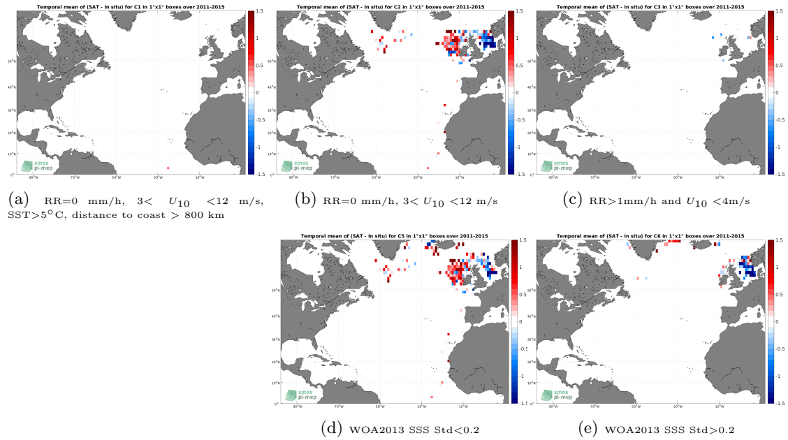
Figure 12: Temporal mean gridded over spatial boxes of size 1^\circ \times 1^\circ of \Delta SSS (Aquarius SSS L2 CAP v5 (JPL) - ICES) for 5 different subdatasets corresponding to:RR=0 mm/h, 3 < U_{10} < 12 m/s, SST >5^\circ\text{C} , distance to coast > 800 km (a), RR=0 mm/h, 3 < U_{10} < 12 m/s (b), RR >1 mm/h and U_{10} < 4 m/s (c), WOA2013 SSS Std <0.2 (d), WOA2013 SSS Std >0.2 (e).
