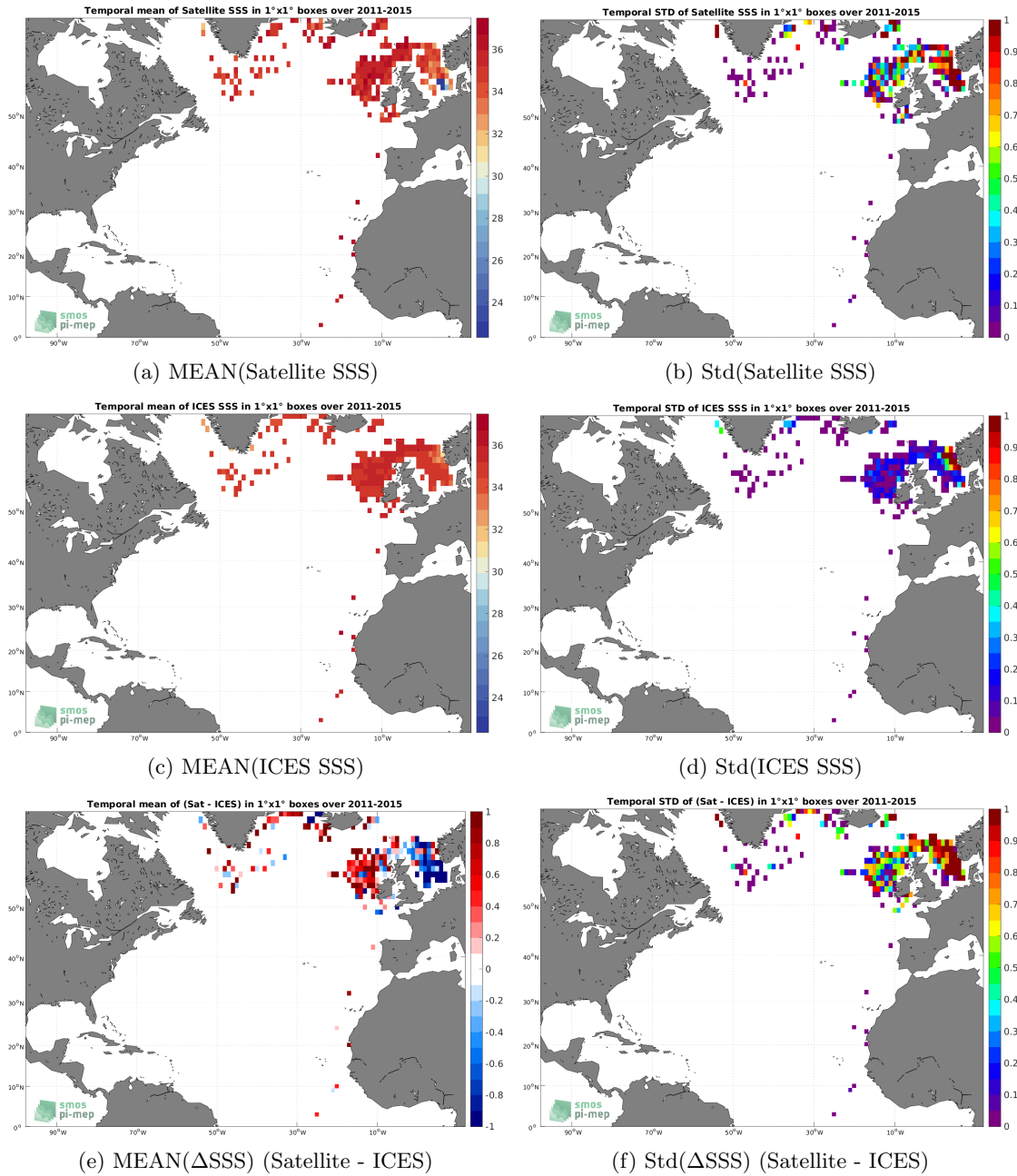
Figure 6: Temporal mean (left) and Std (right) of SSS from Aquarius SSS L2 CAP v5 (JPL) (top), ICES (middle), and of \Delta SSS (Satellite - ICES). Only match-up pairs are used to generate these maps.
