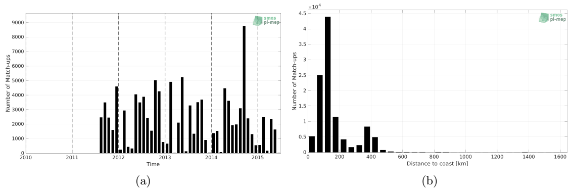
Figure 1: Number of match-ups between ICES and Aquarius SSS L2 CAP v5 (JPL) SSS as a function of time (a) and as function of the distance to coast (b) over the North Atlantic Ocean Pi-MEP region and for the full satellite product period.
