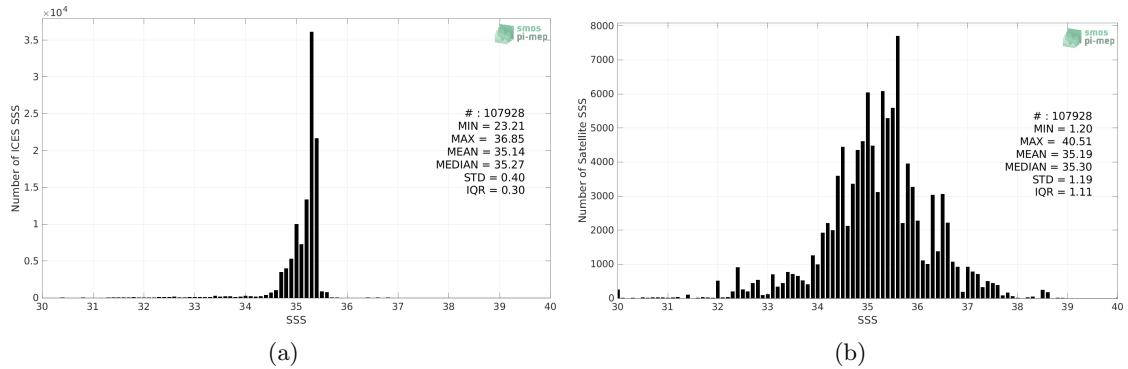
Figure 2: Histograms of SSS from ICES (a) and Aquarius SSS L2 CAP v5 (JPL) (b) considering all match-up pairs per bins of 0.1 over the North Atlantic Ocean Pi-MEP region and for the full satellite product period.
