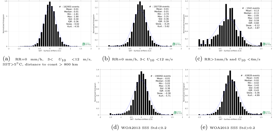
Figure 12: Normalized histogram of \Delta SSS (Aquarius SSS L2 CAP v5 (JPL) - Surface drifters) for 5 different subdatasets corresponding to: RR=0 mm/h, 3 < U_{10} < 12 m/s, SST > 5^\circ\text{C} , distance to coast > 800 km (a), RR=0 mm/h, 3 < U_{10} < 12 m/s (b), RR > 1 mm/h and U_{10} < 4 m/s (c), WOA2013 SSS Std < 0.2 (d), WOA2013 SSS Std > 0.2 (e).
