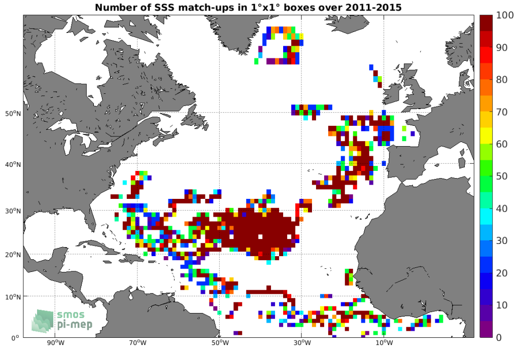
Figure 3: Number of SSS match-ups between Surface drifters SSS and the Aquarius SSS L2 CAP v5 (JPL) SSS product for the North Atlantic Ocean Pi-MEP region over 1°x1° boxes and for the full satellite product period.
