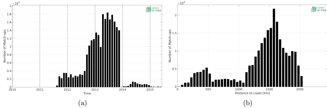
Figure 1: Number of match-ups between Surface drifters and Aquarius-L2-JPL-V5 SSS as a function of time (a) and as function of the distance to coast (b) over the North Atlantic Ocean Pi-MEP region and for the full satellite product period.
