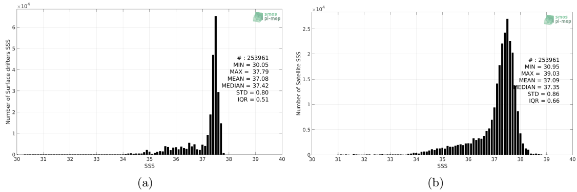
Figure 2: Histograms of SSS from Surface drifters (a) and Aquarius-L2-JPL-V5 (b) considering all match-up pairs per bins of 0.1 over the North Atlantic Ocean Pi-MEP region and for the full satellite product period.
