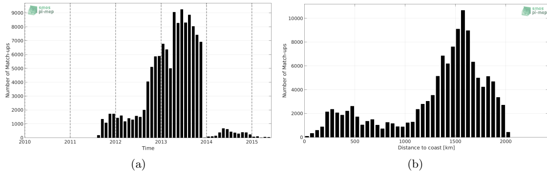
Figure 1: Number of match-ups between Surface drifters and Aquarius-L2-JPL-V5 SSS as a function of time (a) and as function of the distance to coast (b) over the North Atlantic Ocean Pi-MEP region and for the full satellite product period.
