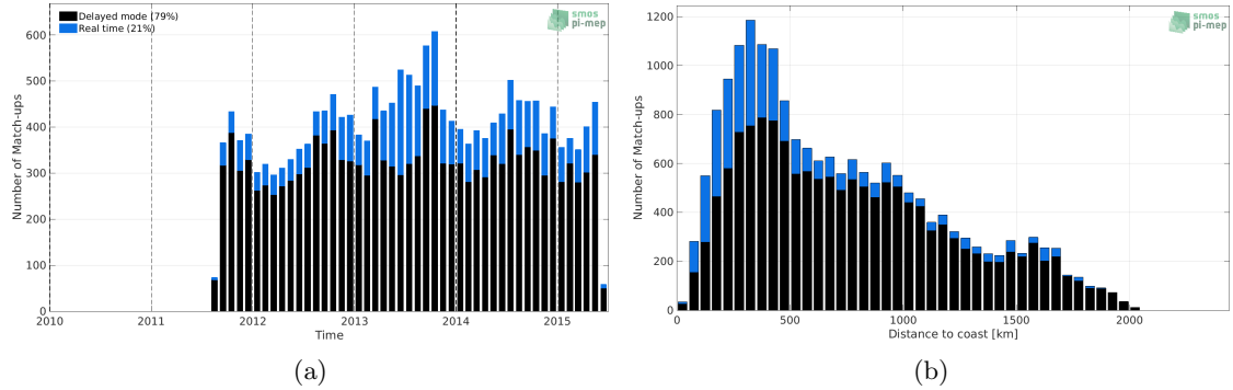
Figure 1: Number of match-ups between Argo and Aquarius SSS L2 CAP v5 (JPL) SSS as a function of time (a) and as function of the distance to coast (b) over the North Atlantic Ocean Pi-MEP region and for the full satellite product period.
