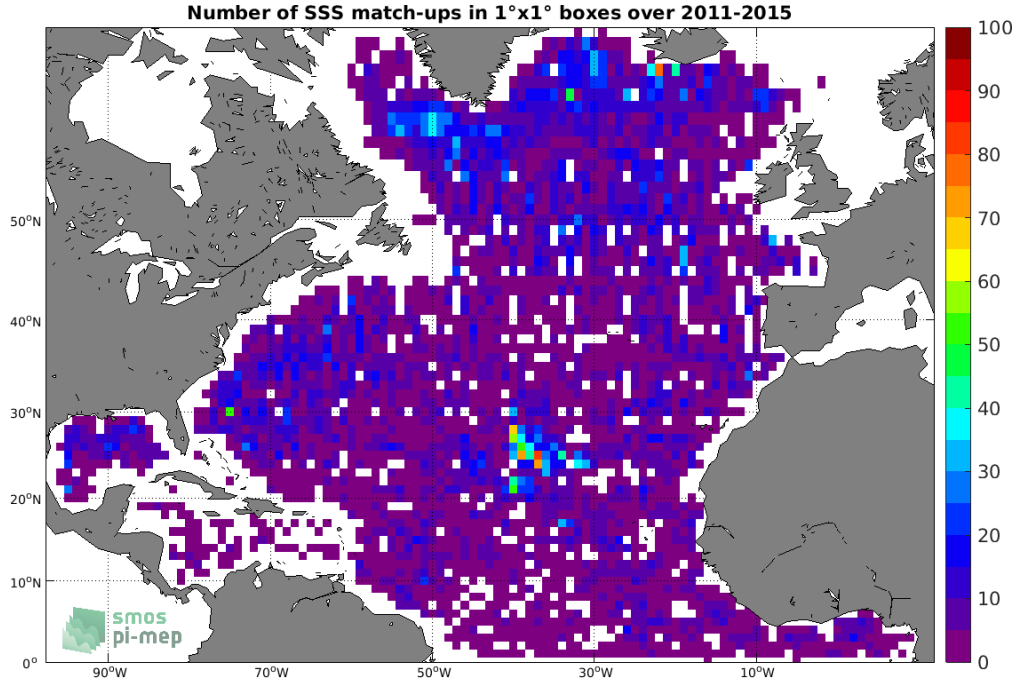
Figure 4: Number of SSS match-ups between Argo SSS and the Aquarius SSS L2 CAP v5 (JPL) SSS product for the North Atlantic Ocean Pi-MEP region over 1^\circ \times 1^\circ boxes and for the full satellite product period.
