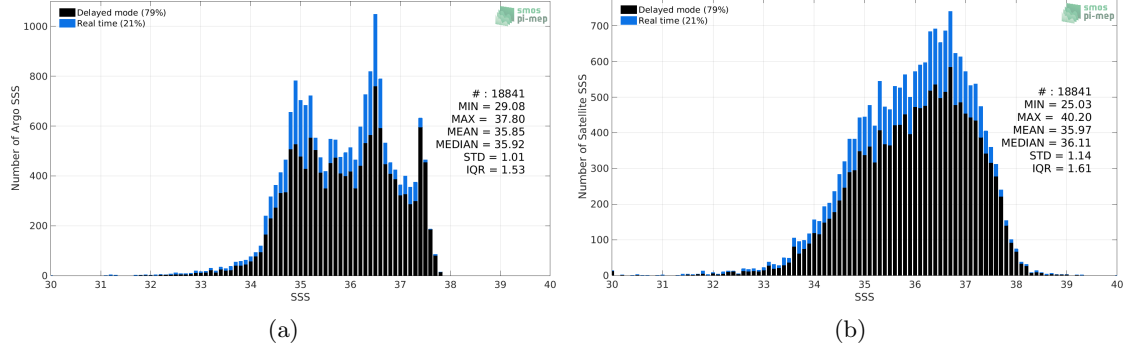
Figure 2: Histograms of SSS from Argo (a) and Aquarius SSS L2 CAP v5 (JPL) (b) considering all match-up pairs per bins of 0.1 over the North Atlantic Ocean Pi-MEP region and for the full satellite product period.
