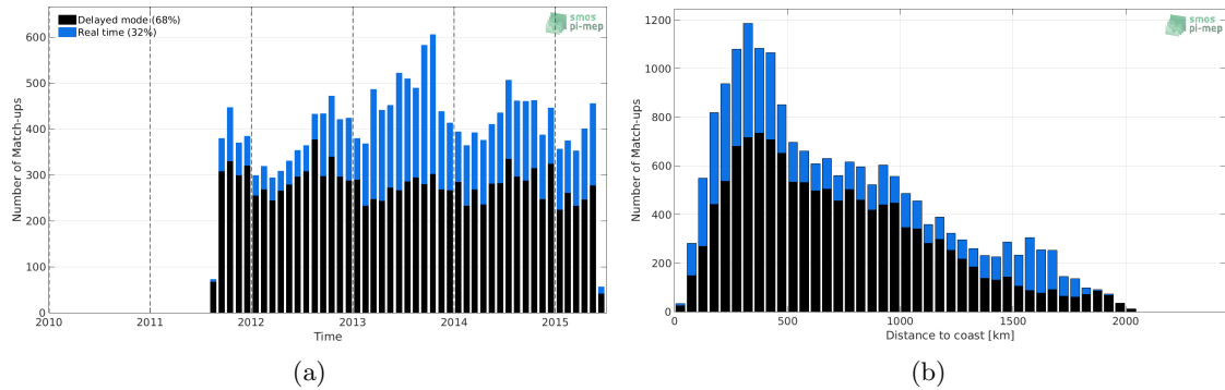
Figure 1: Number of match-ups between Argo and Aquarius-L2-JPL-V5 SSS as a function of time (a) and as function of the distance to coast (b) over the North Atlantic Ocean Pi-MEP region and for the full satellite product period.
