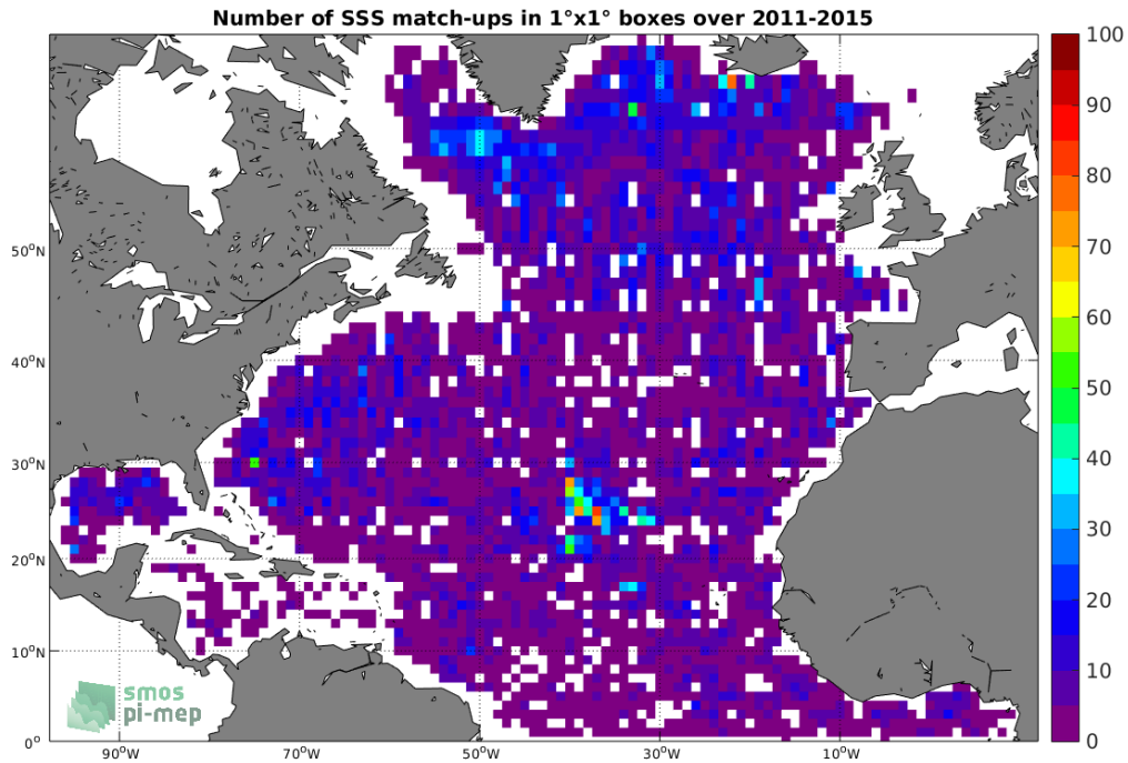
Figure 4: Number of SSS match-ups between Argo SSS and the Aquarius-L2-JPL-V5 SSS product for the North Atlantic Ocean Pi-MEP region over 1^\circ \times 1^\circ boxes and for the full satellite product period.
