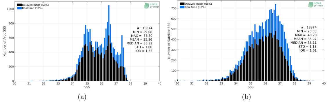
Figure 2: Histograms of SSS from Argo (a) and Aquarius-L2-JPL-V5 (b) considering all match-up pairs per bins of 0.1 over the North Atlantic Ocean Pi-MEP region and for the full satellite product period.
