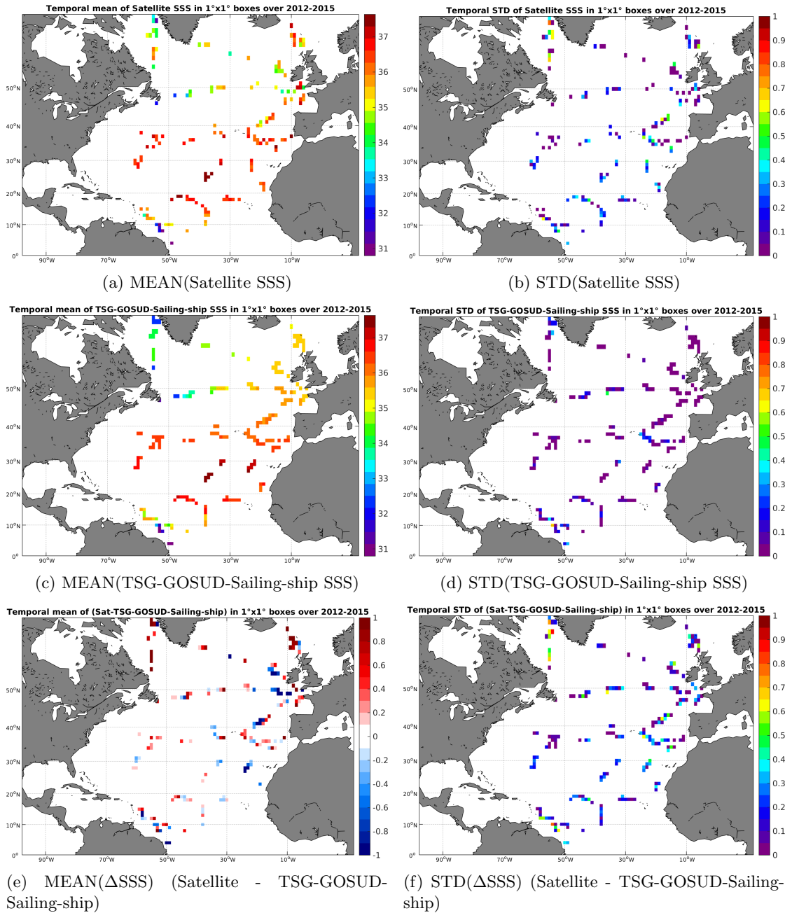
Figure 6: Temporal mean (left) and STD (right) of SSS from AQUARIUS-L2-JPL-V4 (top), TSG-GOSUD-Sailing-ship (middle), and of \Delta SSS (Satellite - TSG-GOSUD-Sailing-ship). Only match-up pairs are used to generate these maps.
