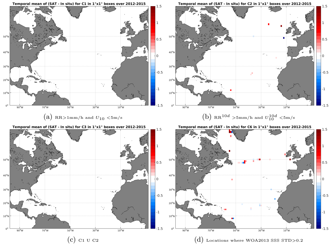
Figure 12: Temporal mean gridded over spatial boxes of size 1^\circ \times 1^\circ of \Delta SSS (AQUARIUS-L2-JPL-V4 - TSG-GOSUD-Sailing-ship) for 4 different subdatasets corresponding to:RR > 1mm/h and U_{10} < 5\text{m/s} (a), RR^{10d} > 5\text{mm/h} and U_{10}^{10d} < 5\text{m/s} (b), C1 U C2 (c),Locations where WOA2013 SSS STD > 0.2 (d).
