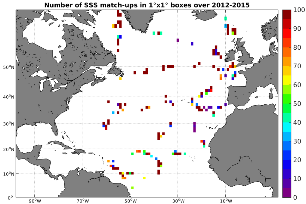
Figure 4: Number of SSS match-ups between TSG-GOSUD-Sailing-ship SSS and the AQUARIUS-L2-JPL-V4 SSS product for the North Atlantic Ocean Pi-MEP region over 1^\circ \times 1^\circ boxes and for the full satellite product period.
