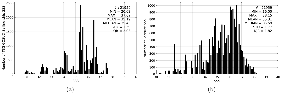
Figure 2: Histograms of SSS from TSG-GOSUD-Sailing-ship (a) and AQUARIUS-L2-JPL-V4 (b) considering all match-up pairs per bins of 0.1 over the North Atlantic Ocean Pi-MEP region and for the full satellite product period.
