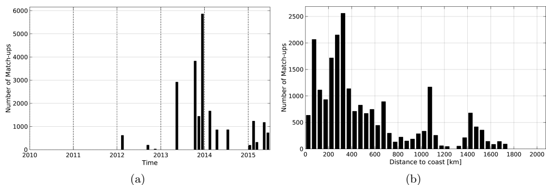
Figure 1: Number of match-ups between TSG-GOSUD-Sailing-ship and AQUARIUS-L2-JPL-V4 SSS as a function of time (a) and as function of the distance to coast (b) over the North Atlantic Ocean Pi-MEP region and for the full satellite product period.
