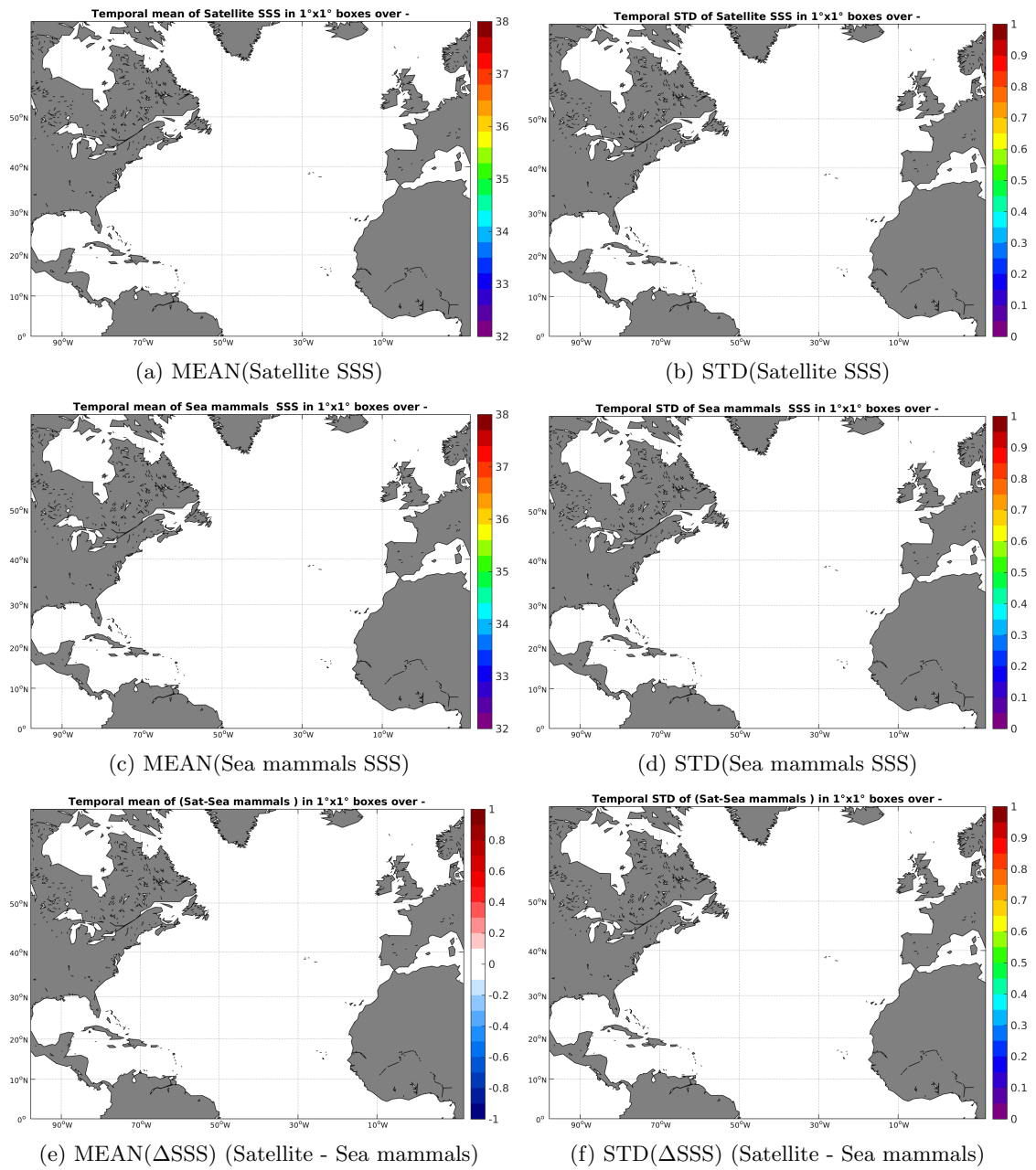
Figure 6: Temporal mean (left) and STD (right) of SSS from AQUARIUS-L2-JPL-V4 (top), Sea mammals (middle), and of \Delta SSS (Satellite - Sea mammals). Only match-up pairs are used to generate these maps.
