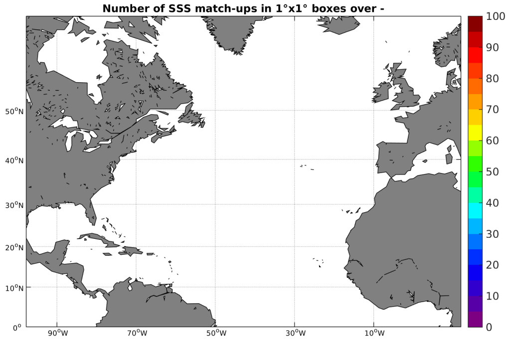
Figure 4: Number of SSS match-ups between Sea mammals SSS and the AQUARIUS-L2-JPL-V4 SSS product for the North Atlantic Ocean Pi-MEP region over 1^\circ \times 1^\circ boxes and for the full satellite product period.
