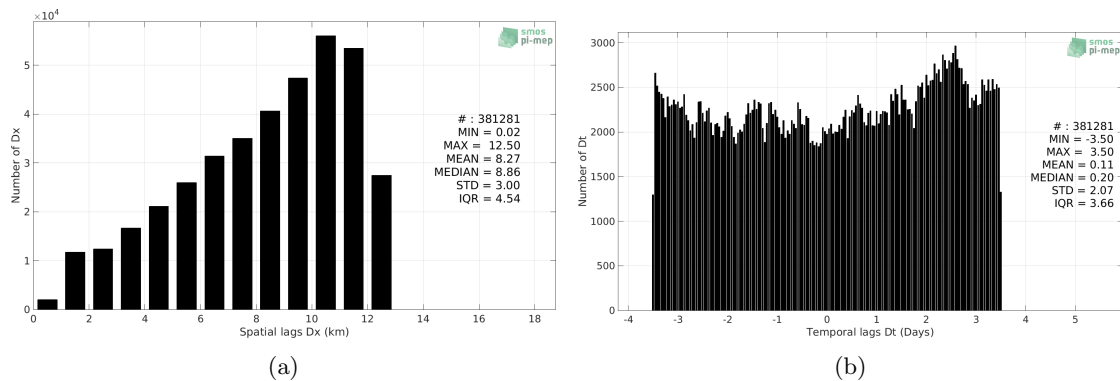
Figure 5: Histograms of the spatial (a) and temporal (b) lags between the location/time of the TSG (GOSUD-Research-vessel) measurement pixel and the date of the corresponding SMOS and SMAP SSS L4 OI v1 - 7 Days (LOPS) SSS pixel.
