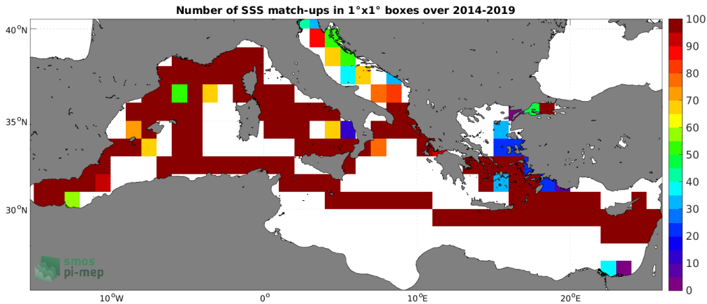
Figure 4: Number of SSS match-ups between TSG (GOSUD-Sailing-ship) SSS and the SMOS SSS L4 v1 - Weekly (CMEMS-CNR) SSS product for the Mediterranean Sea Pi-MEP region over 1^\circ \times 1^\circ boxes and for the full satellite product period.
