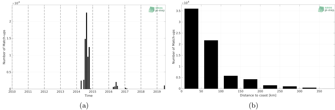
Figure 1: Number of match-ups between TSG (GOSUD-Sailing-ship) and SMOS SSS L4 v1 - Weekly (CMEMS-CNR) SSS as a function of time (a) and as function of the distance to coast (b) over the Mediterranean Sea Pi-MEP region and for the full satellite product period.
