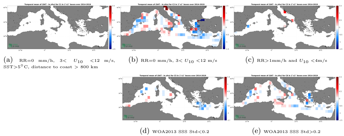
Figure 12: Temporal mean gridded over spatial boxes of size 1^\circ \times 1^\circ of \Delta SSS (SMOS SSS L4 v1 - Weekly (CMEMS-CNR) - TSG (GOSUD-Sailing-ship)) for 5 different subdatasets corresponding to:RR=0 mm/h, 3 < U_{10} < 12 m/s, SST>5°C, distance to coast > 800 km (a), RR=0 mm/h, 3 < U_{10} < 12 m/s (b), RR>1mm/h and U_{10} < 4 m/s (c), WOA2013 SSS Std<0.2 (d), WOA2013 SSS Std>0.2 (e).
