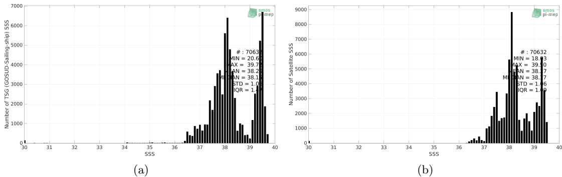
Figure 2: Histograms of SSS from TSG (GOSUD-Sailing-ship) (a) and SMOS SSS L4 v1 - Weekly (CMEMS-CNR) (b) considering all match-up pairs per bins of 0.1 over the Mediterranean Sea Pi-MEP region and for the full satellite product period.
