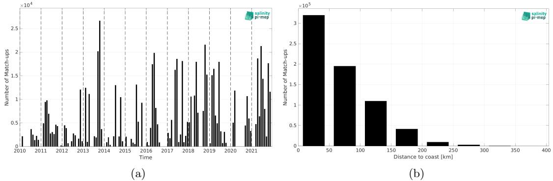
Figure 1: Number of match-ups between TSG (GOSUD-Research-vessel) and SMOS SSS L4 v1 - Weekly (CMEMS-CNR) SSS as a function of time (a) and as function of the distance to coast (b) over the Mediterranean Sea Pi-MEP region and for the full satellite product period.
