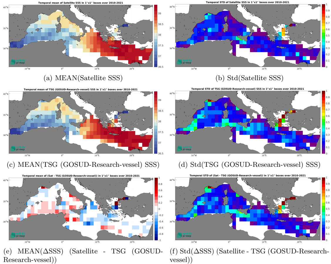
Figure 6: Temporal mean (left) and Std (right) of SSS from SMOS SSS L4 v1 - Weekly (CMEMS-CNR) (top), TSG (GOSUD-Research-vessel) (middle), and of \Delta\text{SSS} (Satellite - TSG (GOSUD-Research-vessel)). Only match-up pairs are used to generate these maps.
