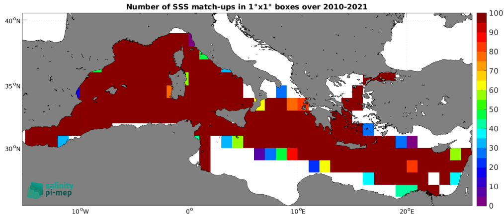
Figure 4: Number of SSS match-ups between TSG (GOSUD-Research-vessel) SSS and the SMOS SSS L4 v1 - Weekly (CMEMS-CNR) SSS product for the Mediterranean Sea Pi-MEP region over 1^\circ \times 1^\circ boxes and for the full satellite product period.
