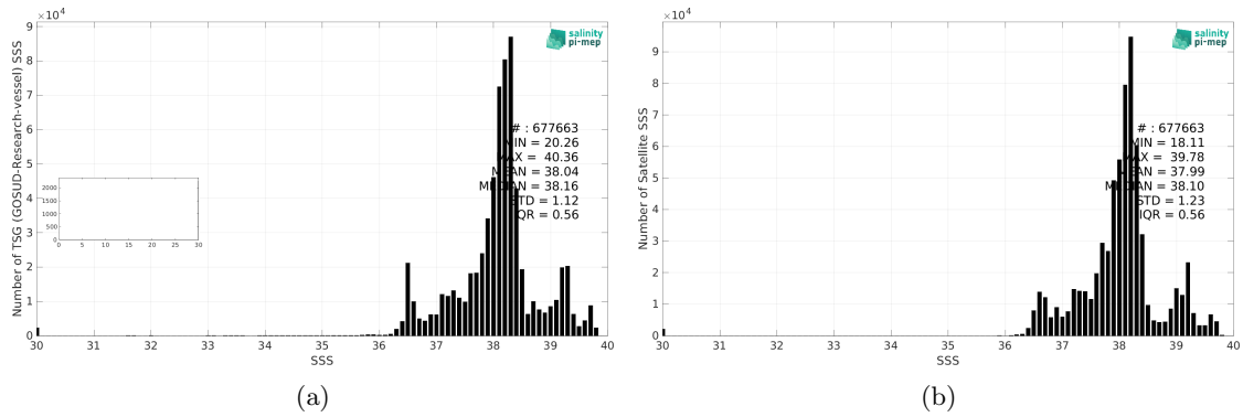
Figure 2: Histograms of SSS from TSG (GOSUD-Research-vessel) (a) and SMOS SSS L4 v1 - Weekly (CMEMS-CNR) (b) considering all match-up pairs per bins of 0.1 over the Mediterranean Sea Pi-MEP region and for the full satellite product period.
