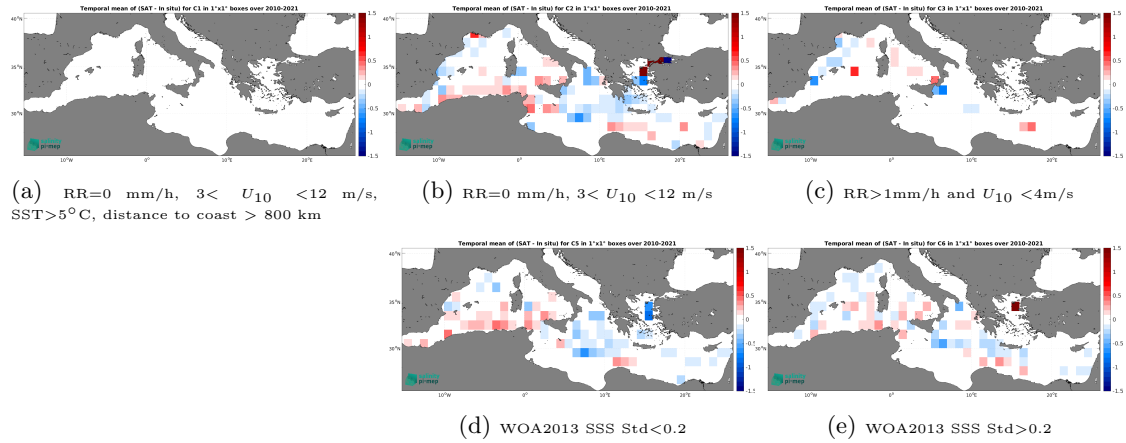
Figure 12: Temporal mean gridded over spatial boxes of size 1^{\circ}\times 1^{\circ} of \Delta SSS (SMOS SSS L4 v1 - Weekly (CMEMS-CNR) - TSG (GOSUD-Research-vessel)) for 5 different subdatasets corresponding to:RR=0 mm/h, 3 < U_{10} < 12 m/s, SST >5^{\circ}\text{C} , distance to coast > 800 km (a), RR=0 mm/h, 3 < U_{10} < 12 m/s (b), RR >1 mm/h and U_{10} < 4 m/s (c), WOA2013 SSS Std <0.2 (d), WOA2013 SSS Std >0.2 (e).
