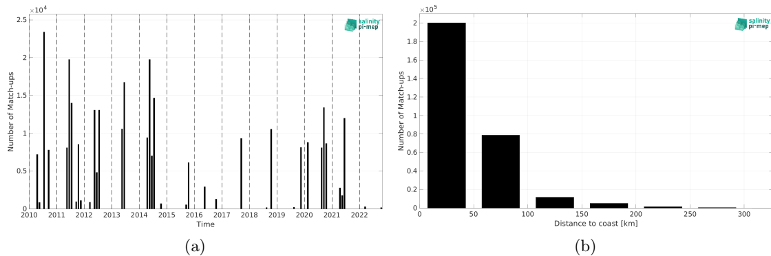
Figure 2: Number of match-ups between TSG (CSIC-UTM) and SMOS SSS L4 v1 - Monthly (CMEMS-CNR) SSS as a function of time (a) and as function of the distance to coast (b) over the Mediterranean Sea Pi-MEP region and for the full satellite product period.
