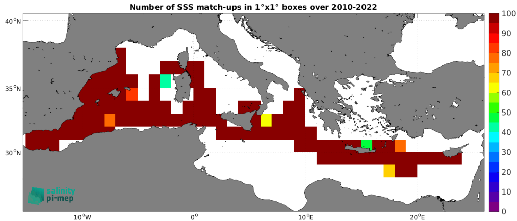
Figure 5: Number of SSS match-ups between TSG (CSIC-UTM) SSS and the SMOS SSS L4 v1 - Monthly (CMEMS-CNR) SSS product for the Mediterranean Sea Pi-MEP region over 1^\circ \times 1^\circ boxes and for the full satellite product period.
