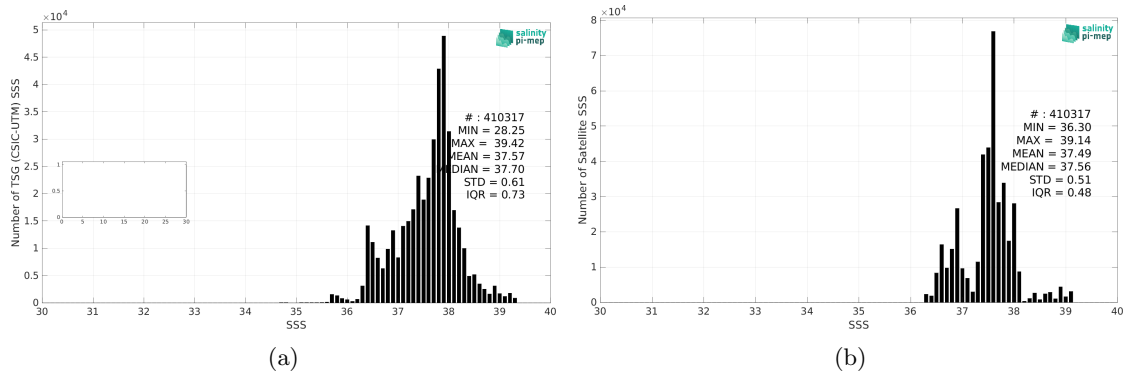
Figure 2: Histograms of SSS from TSG (CSIC-UTM) (a) and SMOS SSS L4 v1 - Monthly (CMEMS-CNR) (b) considering all match-up pairs per bins of 0.1 over the Mediterranean Sea Pi-MEP region and for the full satellite product period.
