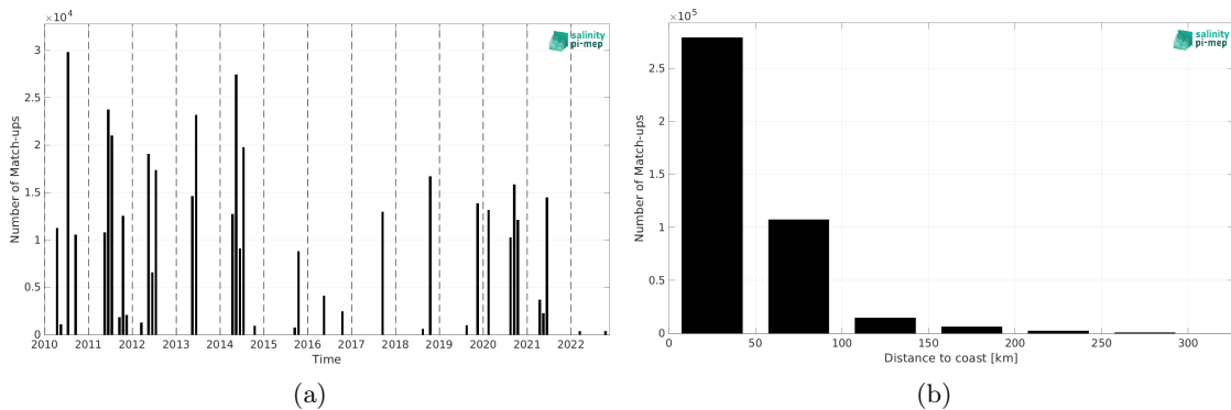
Figure 1: Number of match-ups between TSG (CSIC-UTM) and SMOS SSS L4 v1 - Monthly (CMEMS-CNR) SSS as a function of time (a) and as function of the distance to coast (b) over the Mediterranean Sea Pi-MEP region and for the full satellite product period.
