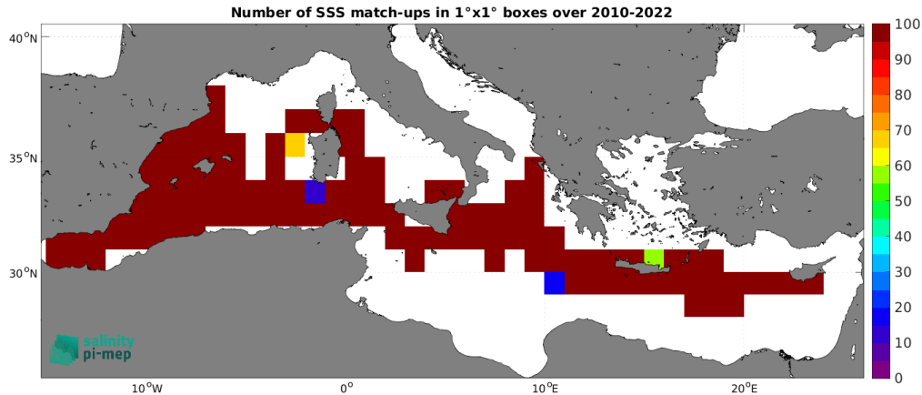
Figure 4: Number of SSS match-ups between TSG (CSIC-UTM) SSS and the SMOS SSS L4 v1 - Monthly (CMEMS-CNR) SSS product for the Mediterranean Sea Pi-MEP region over 1^\circ \times 1^\circ boxes and for the full satellite product period.
