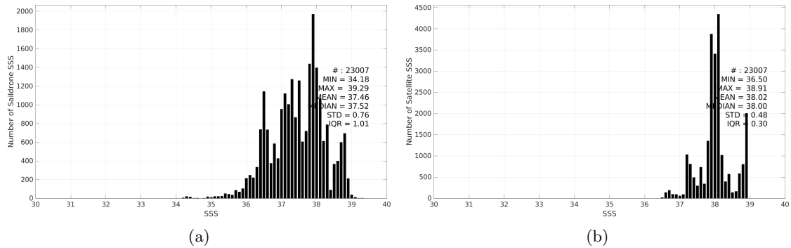
Figure 3: Histograms of SSS from Saildrone (a) and SMOS SSS L4 v1 - Monthly (CMEMS-CNR) (b) considering all match-up pairs per bins of 0.1 over the Mediterranean Sea Pi-MEP region and for the full satellite product period.
