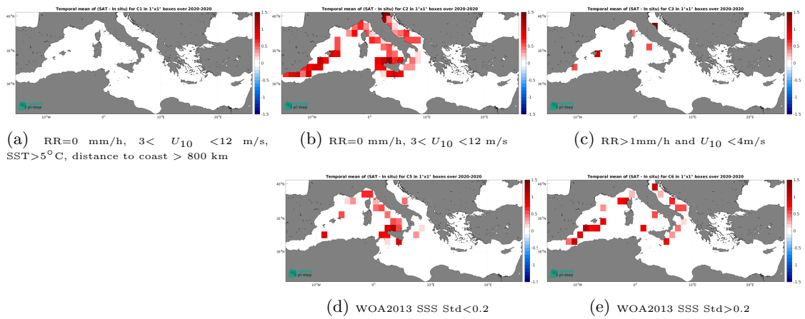
Figure 14: Temporal mean gridded over spatial boxes of size 1^\circ \times 1^\circ of \Delta SSS (SMOS SSS L4 v1 - Monthly (CMEMS-CNR) - Saildrone) for 5 different subdatasets corresponding to:RR=0 mm/h, 3 < U_{10} < 12 m/s, SST>5°C, distance to coast > 800 km (a), RR=0 mm/h, 3 < U_{10} < 12 m/s (b), RR>1mm/h and U_{10} < 4 m/s (c), WOA2013 SSS Std<0.2 (d), WOA2013 SSS Std>0.2 (e).
