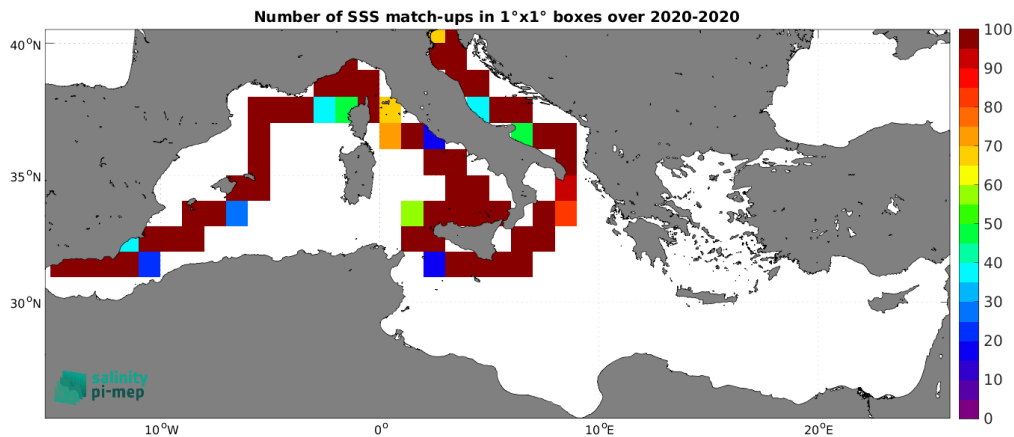
Figure 5: Number of SSS match-ups between Saildrone SSS and the SMOS SSS L4 v1 - Monthly (CMEMS-CNR) SSS product for the Mediterranean Sea Pi-MEP region over 1^\circ \times 1^\circ boxes and for the full satellite product period.
