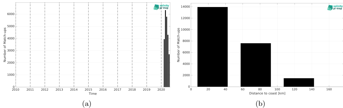
Figure 2: Number of match-ups between Saildrone and SMOS SSS L4 v1 - Monthly (CMEMS-CNR) SSS as a function of time (a) and as function of the distance to coast (b) over the Mediterranean Sea Pi-MEP region and for the full satellite product period.
