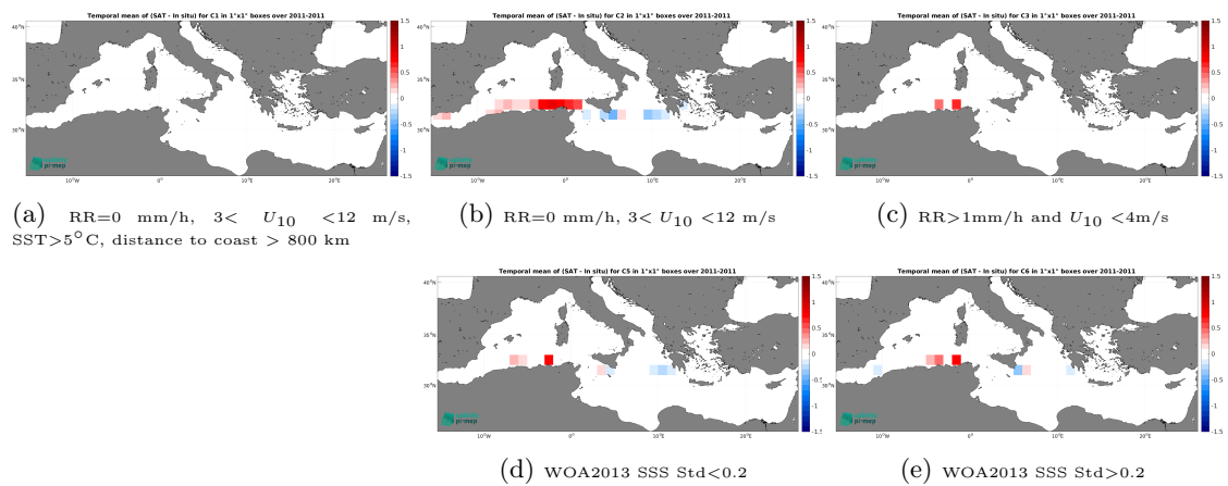
Figure 14: Temporal mean gridded over spatial boxes of size 1^\circ \times 1^\circ of \Delta SSS (SMOS SSS L4 v1 - Daily (CMEMS-CNR) - TSG (SAMOS)) for 5 different subdatasets corresponding to:RR=0 mm/h, 3 < U_{10} < 12 m/s, SST >5^\circ C, distance to coast > 800 km (a), RR=0 mm/h, 3 < U_{10} < 12 m/s (b), RR >1 mm/h and U_{10} < 4 m/s (c), WOA2013 SSS Std <0.2 (d), WOA2013 SSS Std >0.2 (e).
