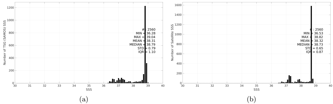
Figure 3: Histograms of SSS from TSG (SAMOS) (a) and SMOS SSS L4 v1 - Daily (CMEMS-CNR) (b) considering all match-up pairs per bins of 0.1 over the Mediterranean Sea Pi-MEP region and for the full satellite product period.
