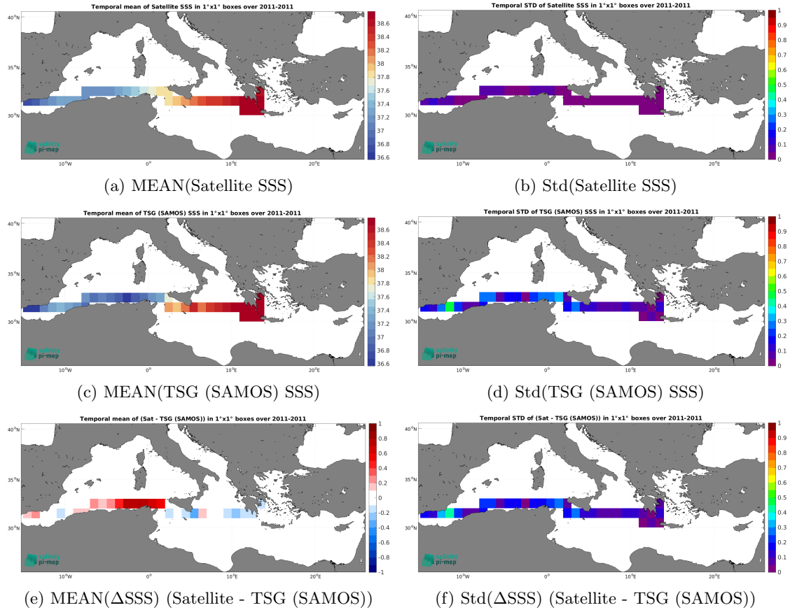
Figure 7: Temporal mean (left) and Std (right) of SSS from SMOS SSS L4 v1 - Daily (CMEMS-CNR) (top), TSG (SAMOS) (middle), and of \Delta\text{SSS} (Satellite - TSG (SAMOS)). Only match-up pairs are used to generate these maps.
