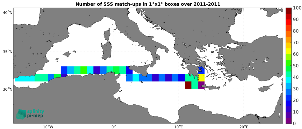
Figure 5: Number of SSS match-ups between TSG (SAMOS) SSS and the SMOS SSS L4 v1 - Daily (CMEMS-CNR) SSS product for the Mediterranean Sea Pi-MEP region over 1^\circ \times 1^\circ boxes and for the full satellite product period.
