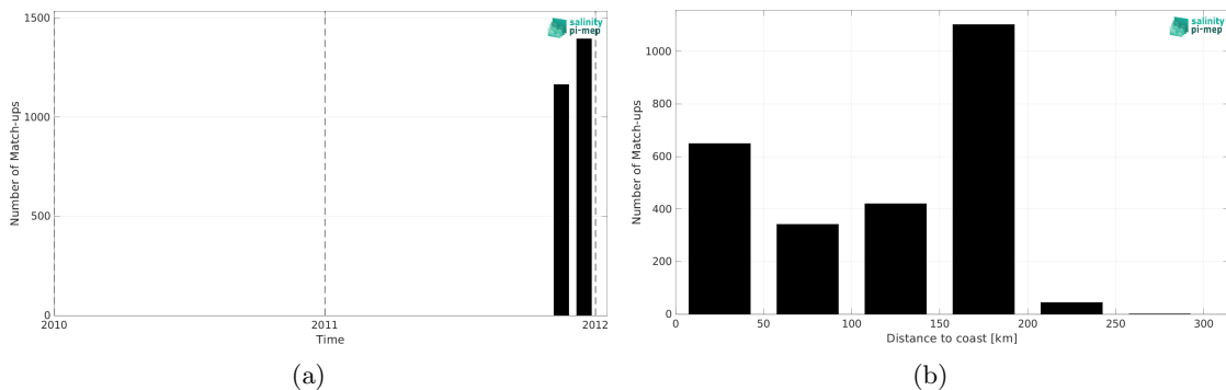
Figure 2: Number of match-ups between TSG (SAMOS) and SMOS SSS L4 v1 - Daily (CMEMS-CNR) SSS as a function of time (a) and as function of the distance to coast (b) over the Mediterranean Sea Pi-MEP region and for the full satellite product period.
