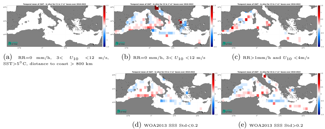
Figure 14: Temporal mean gridded over spatial boxes of size 1^\circ \times 1^\circ of \Delta\text{SSS} (SMOS SSS L4 v1 - Daily (CMEMS-CNR) - TSG (LEGOS-DM)) for 5 different subdatasets corresponding to:RR=0 mm/h, 3 < U_{10} < 12 m/s, SST >5^\circ\text{C} , distance to coast > 800 km (a), RR=0 mm/h, 3 < U_{10} < 12 m/s (b), RR >1 mm/h and U_{10} < 4 m/s (c), WOA2013 SSS Std <0.2 (d), WOA2013 SSS Std >0.2 (e).
