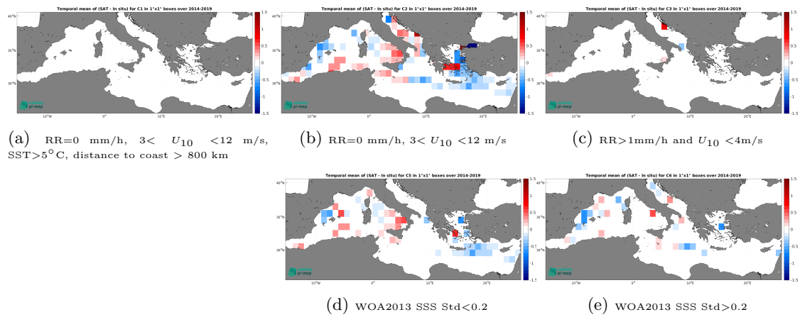
Figure 14: Temporal mean gridded over spatial boxes of size 1^\circ \times 1^\circ of \Delta SSS (SMOS SSS L4 v1 - Daily (CMEMS-CNR) - TSG (GOSUD-Sailing-ship)) for 5 different subdatasets corresponding to:RR=0 mm/h, 3 < U_{10} < 12 m/s, SST>5°C, distance to coast > 800 km (a), RR=0 mm/h, 3 < U_{10} < 12 m/s (b), RR>1mm/h and U_{10} < 4 m/s (c), WOA2013 SSS Std<0.2 (d), WOA2013 SSS Std>0.2 (e).
