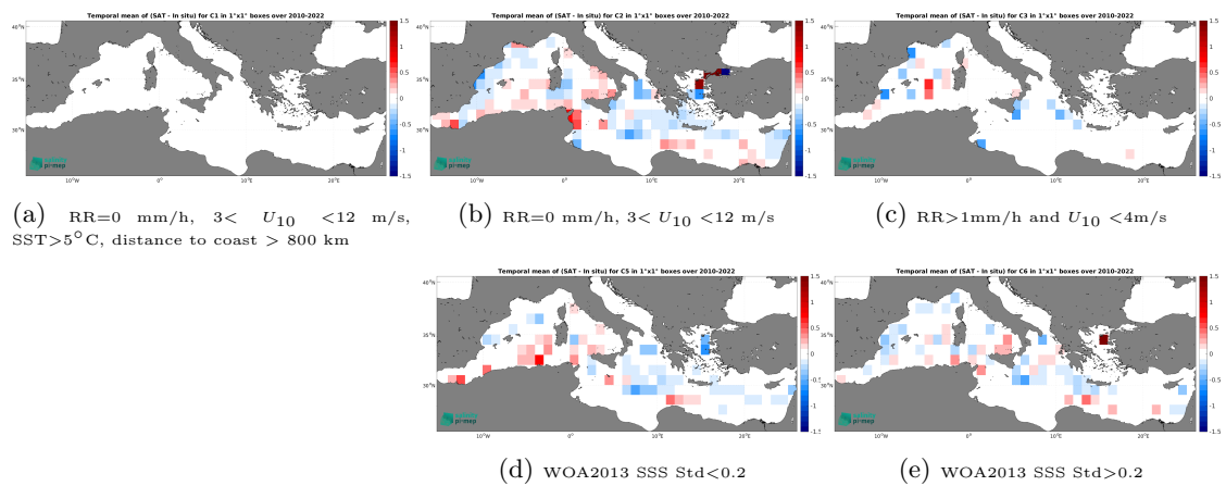
Figure 14: Temporal mean gridded over spatial boxes of size 1^\circ \times 1^\circ of \Delta\text{SSS} (SMOS SSS L4 v1 - Daily (CMEMS-CNR) - TSG (GOSUD-Research-vessel)) for 5 different subdatasets corresponding to:RR=0 mm/h, 3 < U_{10} < 12 m/s, SST>5°C, distance to coast > 800 km (a), RR=0 mm/h, 3 < U_{10} < 12 m/s (b), RR>1mm/h and U_{10} < 4 m/s (c), WOA2013 SSS Std<0.2 (d), WOA2013 SSS Std>0.2 (e).
