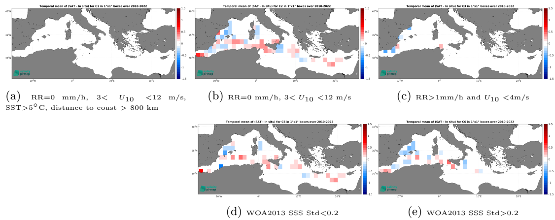
Figure 14: Temporal mean gridded over spatial boxes of size 1^\circ \times 1^\circ of \Delta SSS (SMOS SSS L4 v1 - Daily (CMEMS-CNR) - TSG (CSIC-UTM)) for 5 different subdatasets corresponding to:RR=0 mm/h, 3 < U_{10} < 12 m/s, SST>5°C, distance to coast > 800 km (a), RR=0 mm/h, 3 < U_{10} < 12 m/s (b), RR>1mm/h and U_{10} < 4 m/s (c), WOA2013 SSS Std<0.2 (d), WOA2013 SSS Std>0.2 (e).
