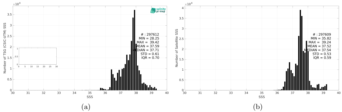
Figure 3: Histograms of SSS from TSG (CSIC-UTM) (a) and SMOS SSS L4 v1 - Daily (CMEMS-CNR) (b) considering all match-up pairs per bins of 0.1 over the Mediterranean Sea Pi-MEP region and for the full satellite product period.
