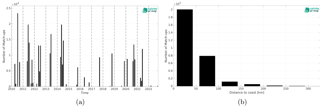
Figure 2: Number of match-ups between TSG (CSIC-UTM) and SMOS SSS L4 v1 - Daily (CMEMS-CNR) SSS as a function of time (a) and as function of the distance to coast (b) over the Mediterranean Sea Pi-MEP region and for the full satellite product period.
