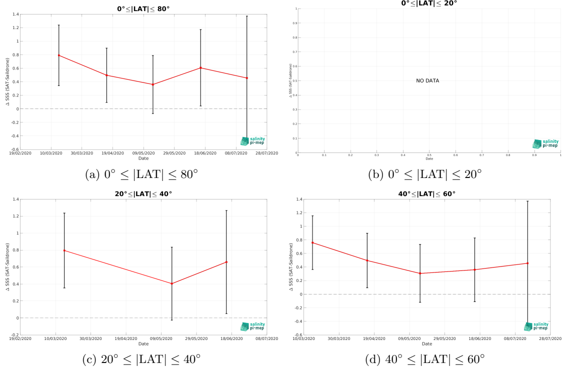
Figure 11: Monthly median (red curves) of \Delta\text{SSS} (Satellite - Saildrone) and \pm 1 Std (black vertical thick bars) as function of time for all the collected Pi-MEP match-up pairs estimated over the Mediterranean Sea Pi-MEP region and for the full satellite product period are shown for different latitude bands: (a) 80°S-80°N, (b) 20°S-20°N, (c) 40°S-20°S and 20°N-40°N and (d) 60°S-40°S and 40°N-60°N.
