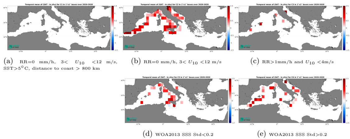
Figure 14: Temporal mean gridded over spatial boxes of size 1^\circ \times 1^\circ of \Delta\text{SSS} (SMOS SSS L4 v1 - Daily (CMEMS-CNR) - Saildrone) for 5 different subdatasets corresponding to:RR=0 mm/h, 3 < U_{10} < 12 m/s, SST>5°C, distance to coast > 800 km (a), RR=0 mm/h, 3 < U_{10} < 12 m/s (b), RR>1mm/h and U_{10} < 4 m/s (c), WOA2013 SSS Std<0.2 (d), WOA2013 SSS Std>0.2 (e).
