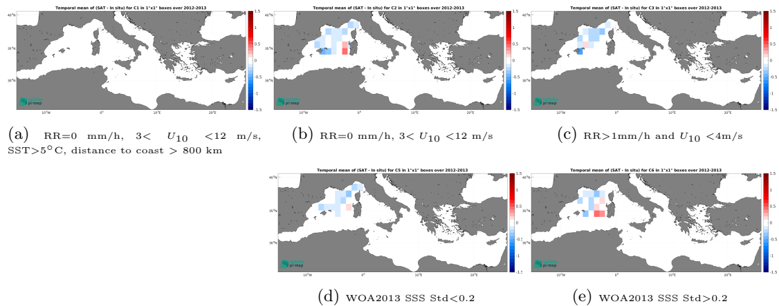
Figure 13: Temporal mean gridded over spatial boxes of size 1^\circ \times 1^\circ of \Delta SSS (SMOS SSS L4 v1 - Daily (CMEMS-CNR) - Surface drifters) for 5 different subdatasets corresponding to:RR=0 mm/h, 3 < U_{10} < 12 m/s, SST >5^\circ C, distance to coast > 800 km (a), RR=0 mm/h, 3 < U_{10} < 12 m/s (b), RR >1 mm/h and U_{10} < 4 m/s (c), WOA2013 SSS Std <0.2 (d), WOA2013 SSS Std >0.2 (e).
