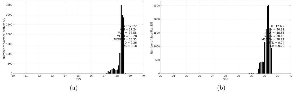
Figure 3: Histograms of SSS from Surface drifters (a) and SMOS SSS L4 v1 - Daily (CMEMS-CNR) (b) considering all match-up pairs per bins of 0.1 over the Mediterranean Sea Pi-MEP region and for the full satellite product period.
