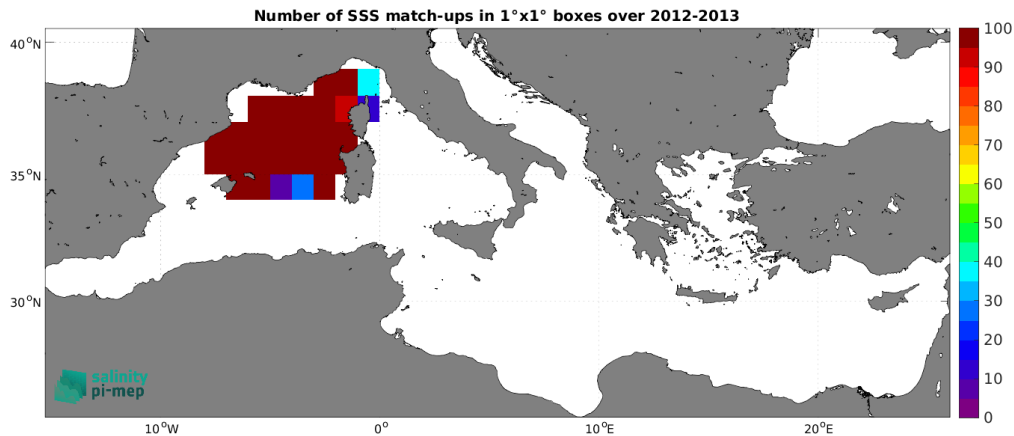
Figure 4: Number of SSS match-ups between Surface drifters SSS and the SMOS SSS L4 v1 - Daily (CMEMS-CNR) SSS product for the Mediterranean Sea Pi-MEP region over 1^\circ \times 1^\circ boxes and for the full satellite product period.
