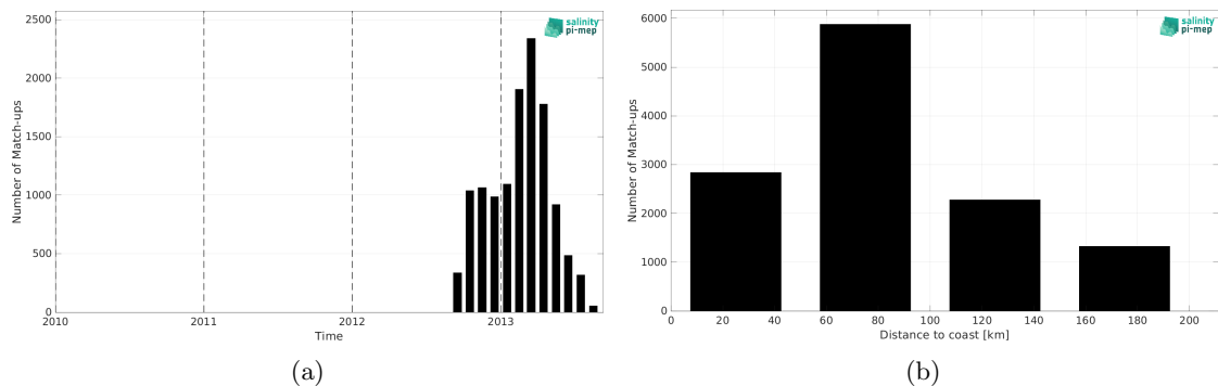
Figure 2: Number of match-ups between Surface drifters and SMOS SSS L4 v1 - Daily (CMEMS-CNR) SSS as a function of time (a) and as function of the distance to coast (b) over the Mediterranean Sea Pi-MEP region and for the full satellite product period.
