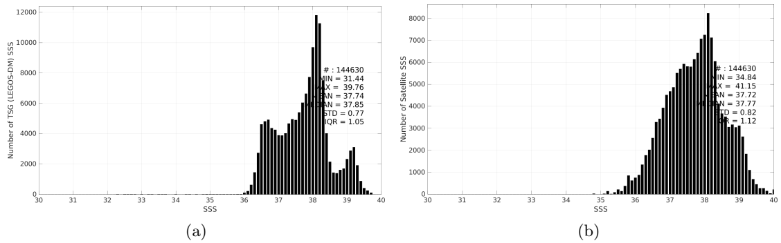
Figure 3: Histograms of SSS from TSG (LEGOS-DM) (a) and SMOS SSS L4 OI v346 - Weekly (CMEMS-CATDS-LOPS) (b) considering all match-up pairs per bins of 0.1 over the Mediterranean Sea Pi-MEP region and for the full satellite product period.
