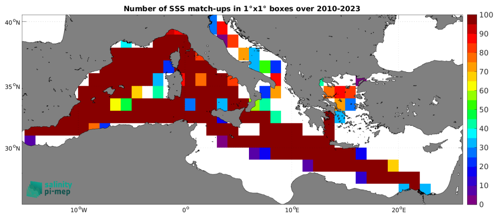
Figure 5: Number of SSS match-ups between TSG (LEGOS-DM) SSS and the SMOS SSS L4 OI v346 - Weekly (CMEMS-CATDS-LOPS) SSS product for the Mediterranean Sea Pi-MEP region over 1^\circ \times 1^\circ boxes and for the full satellite product period.
