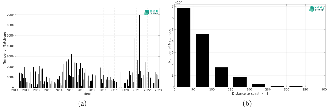
Figure 2: Number of match-ups between TSG (LEGOS-DM) and SMOS SSS L4 OI v346 - Weekly (CMEMS-CATDS-LOPS) SSS as a function of time (a) and as function of the distance to coast (b) over the Mediterranean Sea Pi-MEP region and for the full satellite product period.
