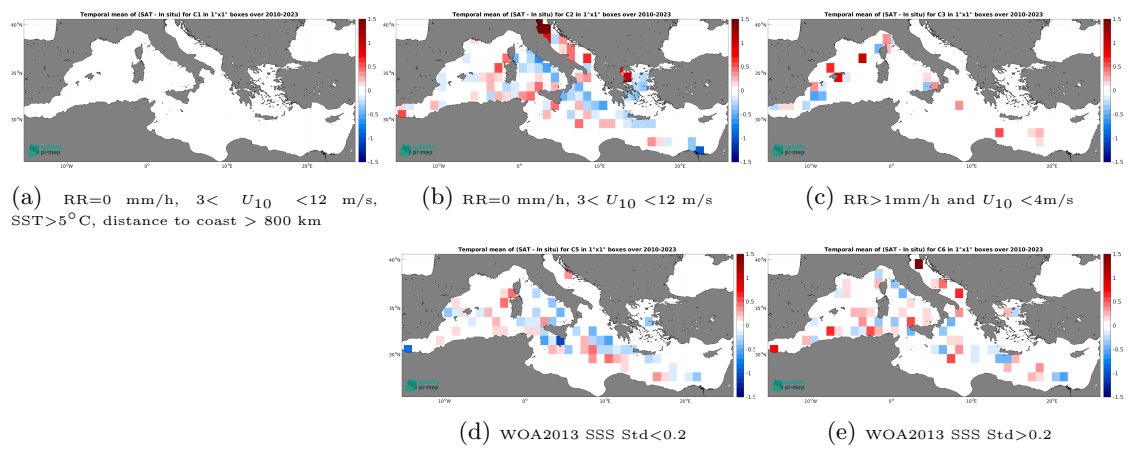
Figure 14: Temporal mean gridded over spatial boxes of size 1^\circ \times 1^\circ of \Delta SSS (SMOS SSS L4 OI v346 - Weekly (CMEMS-CATDS-LOPS) - TSG (LEGOS-DM)) for 5 different subdatasets corresponding to:RR=0 mm/h, 3 < U_{10} < 12 m/s, SST >5^\circ\text{C} , distance to coast > 800 km (a), RR=0 mm/h, 3 < U_{10} < 12 m/s (b), RR >1 mm/h and U_{10} < 4 m/s (c), WOA2013 SSS Std <0.2 (d), WOA2013 SSS Std >0.2 (e).
