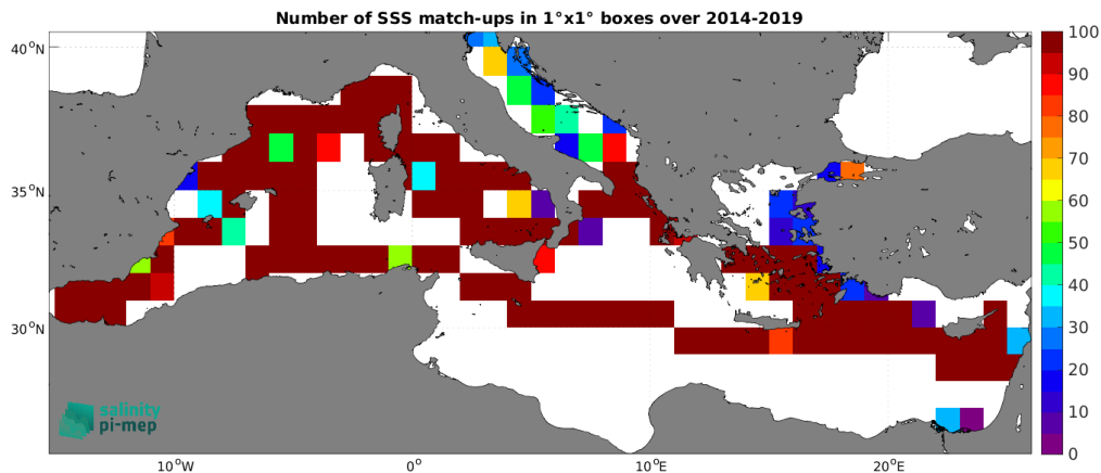
Figure 5: Number of SSS match-ups between TSG (GOSUD-Sailing-ship) SSS and the SMOS SSS L4 OI v346 - Weekly (CMEMS-CATDS-LOPS) SSS product for the Mediterranean Sea Pi-MEP region over 1^\circ \times 1^\circ boxes and for the full satellite product period.
