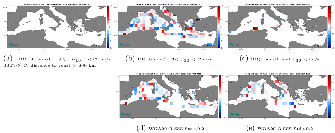
Figure 14: Temporal mean gridded over spatial boxes of size 1^\circ \times 1^\circ of \Delta SSS (SMOS SSS L4 OI v346 - Weekly (CMEMS-CATDS-LOPS) - TSG (GOSUD-Sailing-ship)) for 5 different sub-datasets corresponding to:RR=0 mm/h, 3 < U_{10} < 12 m/s, SST >5^\circ\text{C} , distance to coast > 800 km (a), RR=0 mm/h, 3 < U_{10} < 12 m/s (b), RR >1 mm/h and U_{10} < 4 m/s (c), WOA2013 SSS Std <0.2 (d), WOA2013 SSS Std >0.2 (e).
