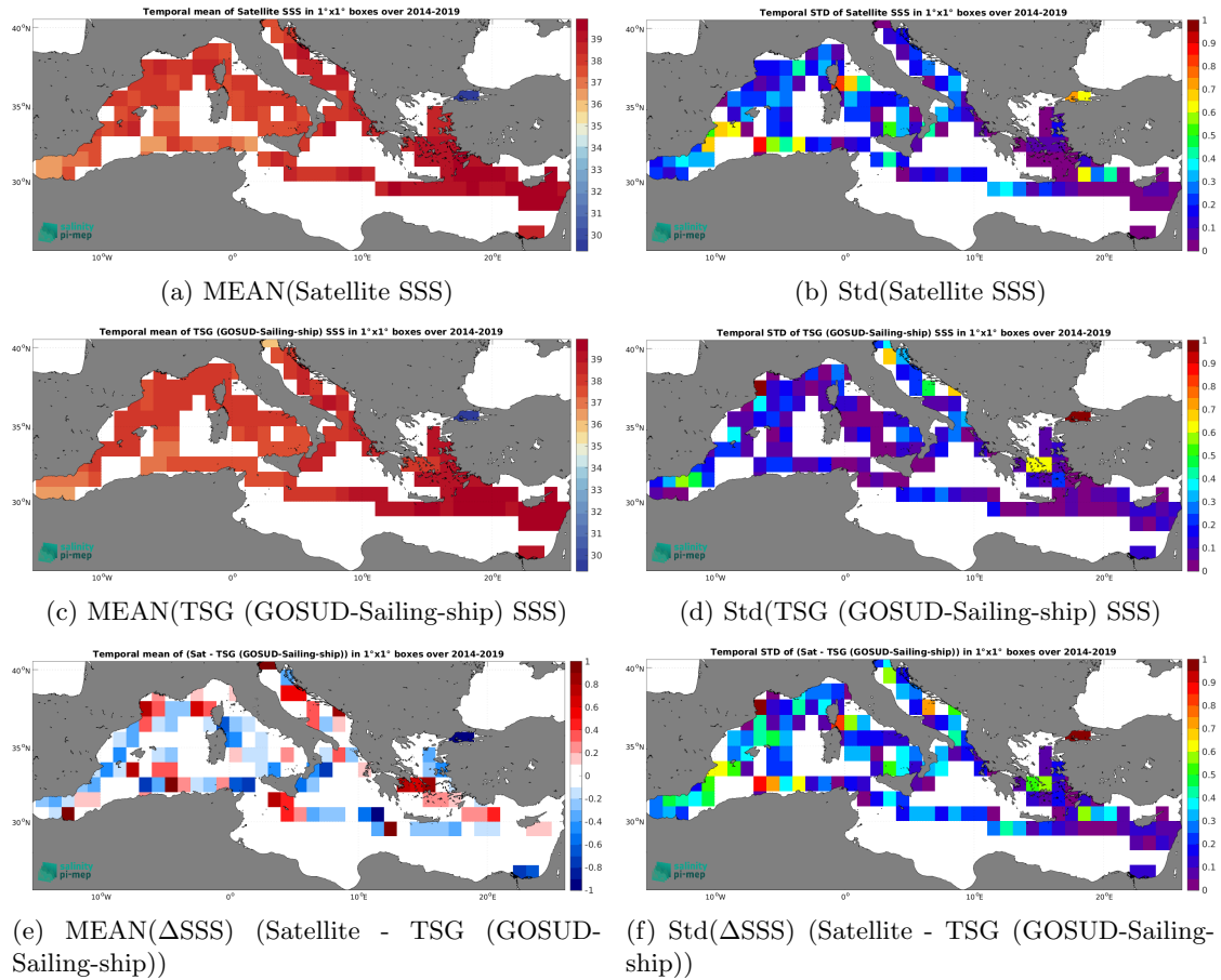
Figure 7: Temporal mean (left) and Std (right) of SSS from SMOS SSS L4 OI v346 - Weekly (CMEMS-CATDS-LOPS) (top), TSG (GOSUD-Sailing-ship) (middle), and of \Delta SSS (Satellite - TSG (GOSUD-Sailing-ship)). Only match-up pairs are used to generate these maps.
