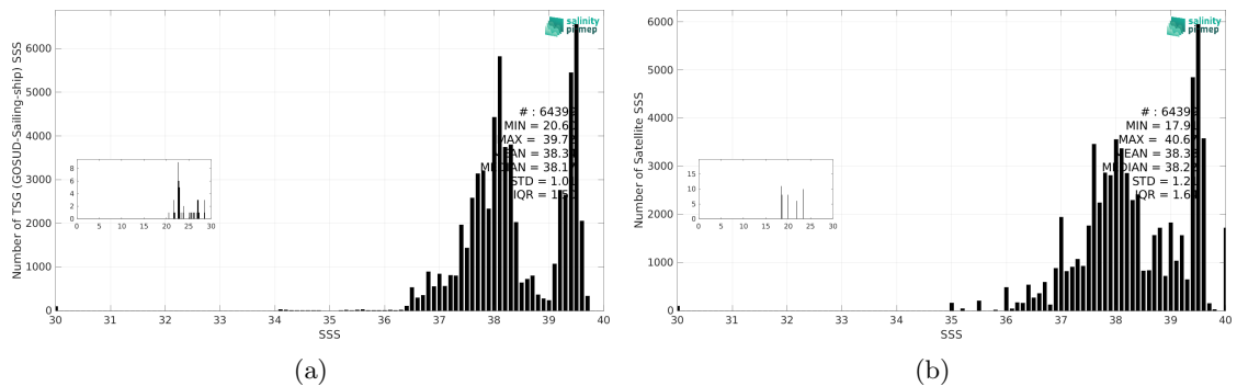
Figure 3: Histograms of SSS from TSG (GOSUD-Sailing-ship) (a) and SMOS SSS L4 OI v346 - Weekly (CMEMS-CATDS-LOPS) (b) considering all match-up pairs per bins of 0.1 over the Mediterranean Sea Pi-MEP region and for the full satellite product period.
