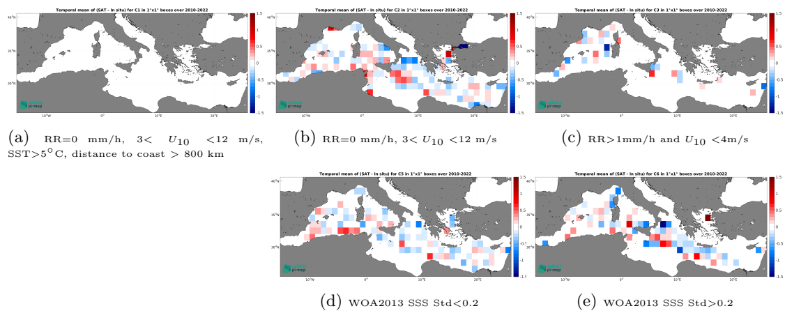
Figure 14: Temporal mean gridded over spatial boxes of size 1^\circ \times 1^\circ of \Delta SSS (SMOS SSS L4 OI v346 - Weekly (CMEMS-CATDS-LOPS) - TSG (GOSUD-Research-vessel)) for 5 different subdatasets corresponding to:RR=0 mm/h, 3 < U_{10} < 12 m/s, SST >5^\circ\text{C} , distance to coast > 800 km (a), RR=0 mm/h, 3 < U_{10} < 12 m/s (b), RR >1 mm/h and U_{10} < 4 m/s (c), WOA2013 SSS Std <0.2 (d), WOA2013 SSS Std >0.2 (e).
