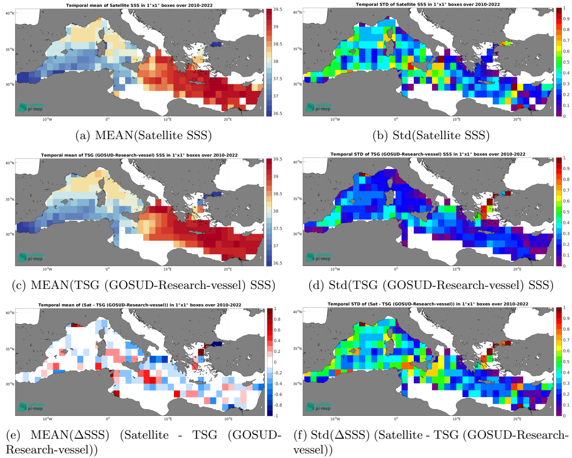
Figure 7: Temporal mean (left) and Std (right) of SSS from SMOS SSS L4 OI v346 - Weekly (CMEMS-CATDS-LOPS) (top), TSG (GOSUD-Research-vessel) (middle), and of \Delta SSS (Satellite - TSG (GOSUD-Research-vessel)). Only match-up pairs are used to generate these maps.
