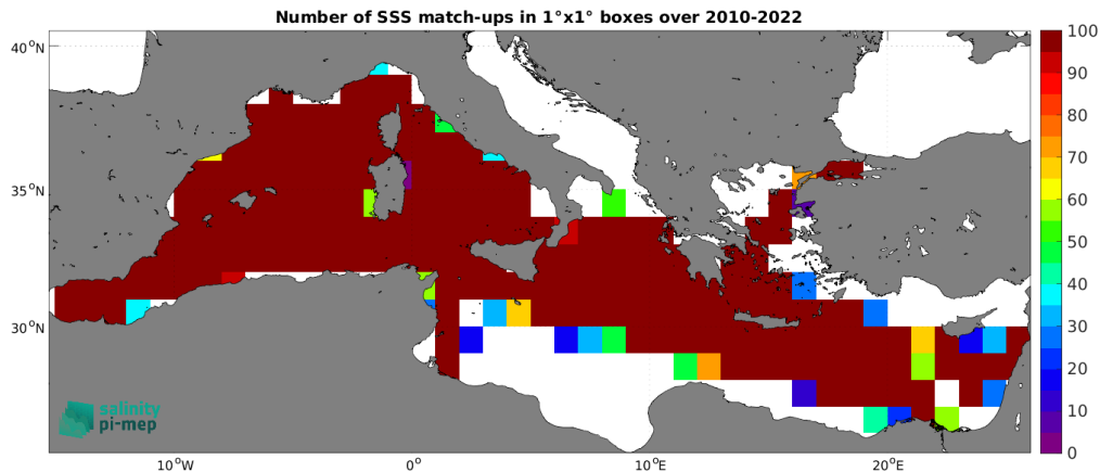
Figure 5: Number of SSS match-ups between TSG (GOSUD-Research-vessel) SSS and the SMOS SSS L4 OI v346 - Weekly (CMEMS-CATDS-LOPS) SSS product for the Mediterranean Sea Pi-MEP region over 1^\circ \times 1^\circ boxes and for the full satellite product period.
