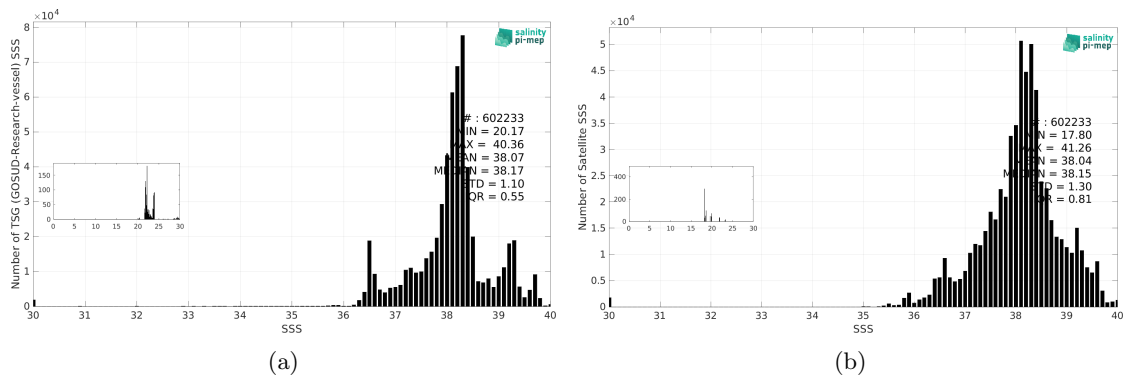
Figure 3: Histograms of SSS from TSG (GOSUD-Research-vessel) (a) and SMOS SSS L4 OI v346 - Weekly (CMEMS-CATDS-LOPS) (b) considering all match-up pairs per bins of 0.1 over the Mediterranean Sea Pi-MEP region and for the full satellite product period.
