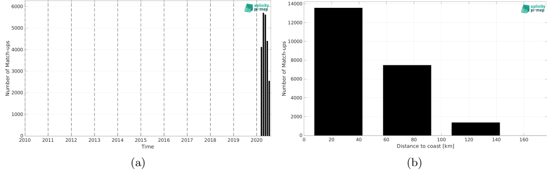
Figure 2: Number of match-ups between Saildrone and SMOS SSS L4 OI v346 - Weekly (CMEMS-CATDS-LOPS) SSS as a function of time (a) and as function of the distance to coast (b) over the Mediterranean Sea Pi-MEP region and for the full satellite product period.
