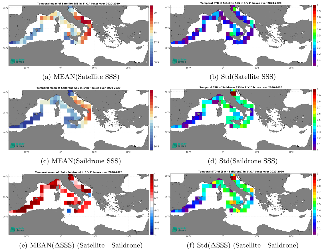
Figure 7: Temporal mean (left) and Std (right) of SSS from SMOS SSS L4 OI v346 - Weekly (CMEMS-CATDS-LOPS) (top), Saildrone (middle), and of \Delta SSS (Satellite - Saildrone). Only match-up pairs are used to generate these maps.
