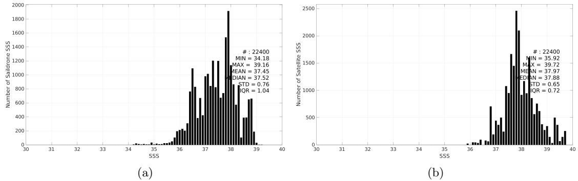
Figure 3: Histograms of SSS from Saildrone (a) and SMOS SSS L4 OI v346 - Weekly (CMEMS-CATDS-LOPS) (b) considering all match-up pairs per bins of 0.1 over the Mediterranean Sea Pi-MEP region and for the full satellite product period.
