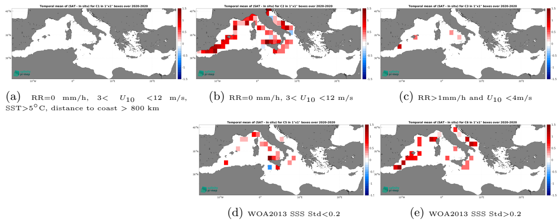
Figure 14: Temporal mean gridded over spatial boxes of size 1^\circ \times 1^\circ of \Delta SSS (SMOS SSS L4 OI v346 - Weekly (CMEMS-CATDS-LOPS) - Saildrone) for 5 different subdatasets corresponding to:RR=0 mm/h, 3 < U_{10} < 12 m/s, SST>5°C, distance to coast > 800 km (a), RR=0 mm/h, 3 < U_{10} < 12 m/s (b), RR>1mm/h and U_{10} < 4 m/s (c), WOA2013 SSS Std<0.2 (d), WOA2013 SSS Std>0.2 (e).
