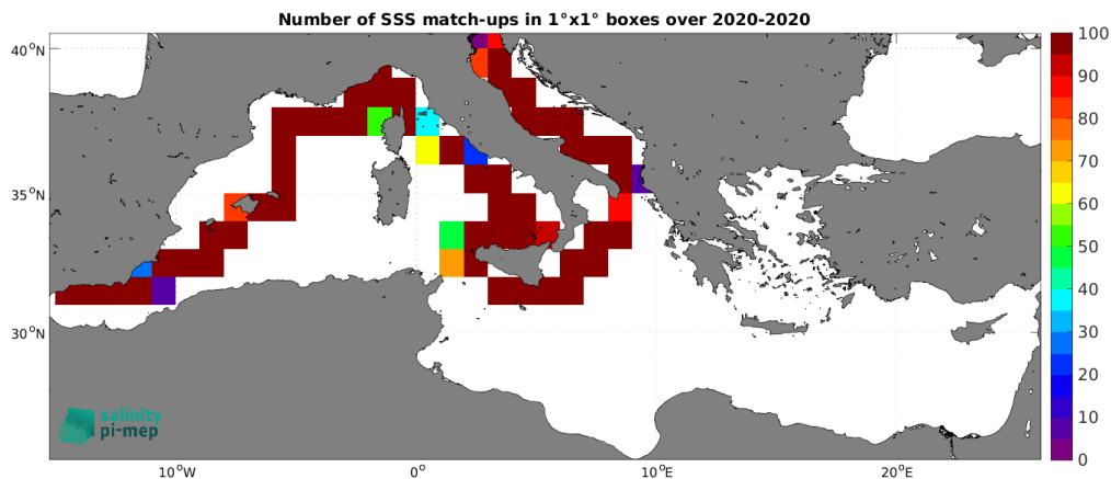
Figure 5: Number of SSS match-ups between Saildrone SSS and the SMOS SSS L4 OI v346 - Weekly (CMEMS-CATDS-LOPS) SSS product for the Mediterranean Sea Pi-MEP region over 1^\circ \times 1^\circ boxes and for the full satellite product period.
