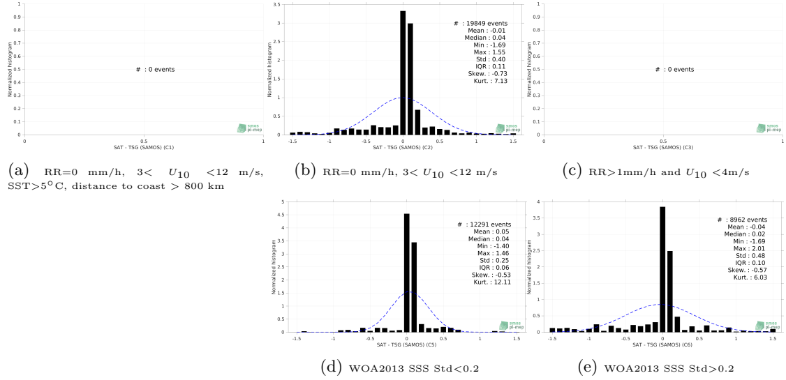
Figure 13: Normalized histogram of \Delta SSS (SMOS SSS L4 OI v342 - Weekly (CMEMS-CATDS-LOPS) - TSG (SAMOS)) for 5 different subdatasets corresponding to: RR=0 mm/h, 3 < U_{10} < 12 m/s, SST >5^{\circ} C, distance to coast > 800 km (a), RR=0 mm/h, 3 < U_{10} < 12 m/s (b), RR >1 mm/h and U_{10} < 4 m/s (c), WOA2013 SSS Std <0.2 (d), WOA2013 SSS Std >0.2 (e).
