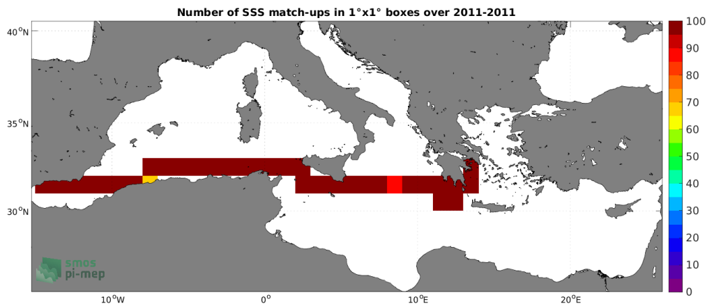
Figure 4: Number of SSS match-ups between TSG (SAMOS) SSS and the SMOS SSS L4 OI v342 - Weekly (CMEMS-CATDS-LOPS) SSS product for the Mediterranean Sea Pi-MEP region over 1^\circ \times 1^\circ boxes and for the full satellite product period.
