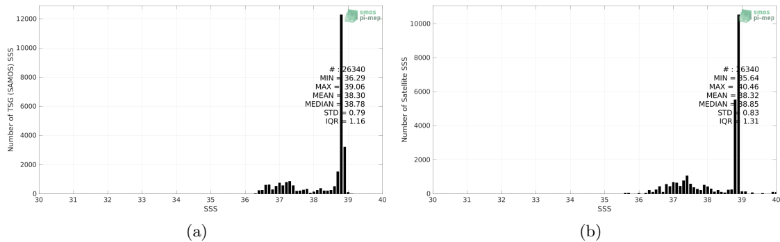
Figure 2: Histograms of SSS from TSG (SAMOS) (a) and SMOS SSS L4 OI v342 - Weekly (CMEMS-CATDS-LOPS) (b) considering all match-up pairs per bins of 0.1 over the Mediterranean Sea Pi-MEP region and for the full satellite product period.
