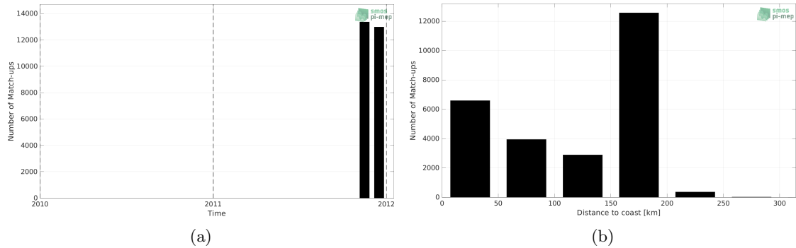
Figure 1: Number of match-ups between TSG (SAMOS) and SMOS SSS L4 OI v342 - Weekly (CMEMS-CATDS-LOPS) SSS as a function of time (a) and as function of the distance to coast (b) over the Mediterranean Sea Pi-MEP region and for the full satellite product period.
