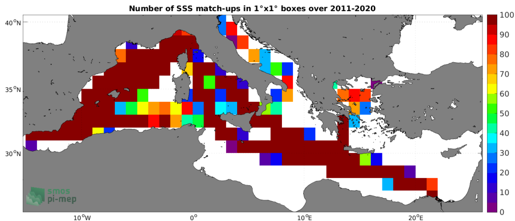
Figure 4: Number of SSS match-ups between TSG (LEGOS-DM) SSS and the SMOS SSS L4 OI v342 - Weekly (CMEMS-CATDS-LOPS) SSS product for the Mediterranean Sea Pi-MEP region over 1^\circ \times 1^\circ boxes and for the full satellite product period.
