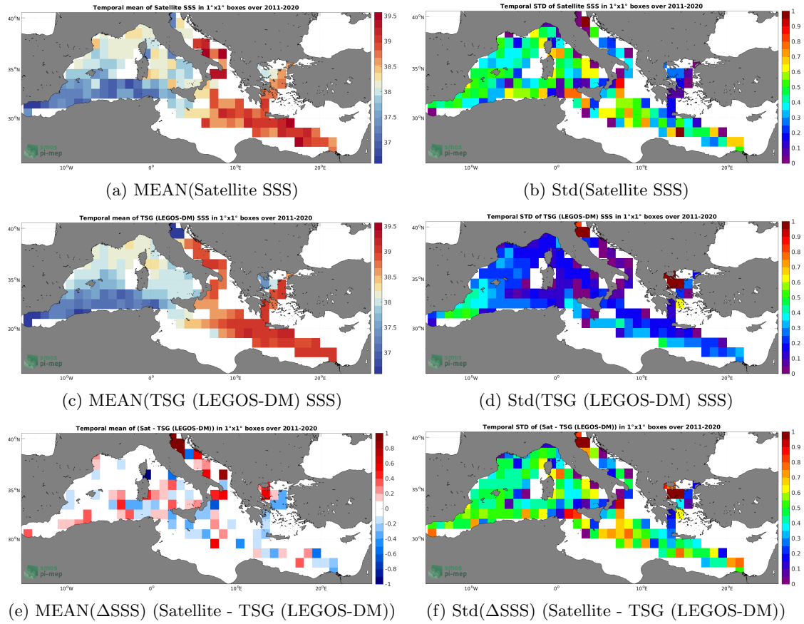
Figure 6: Temporal mean (left) and Std (right) of SSS from SMOS SSS L4 OI v342 - Weekly (CMEMS-CATDS-LOPS) (top), TSG (LEGOS-DM) (middle), and of \Delta SSS (Satellite - TSG (LEGOS-DM)). Only match-up pairs are used to generate these maps.
