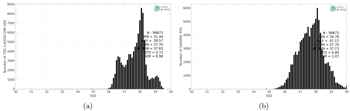
Figure 2: Histograms of SSS from TSG (LEGOS-DM) (a) and SMOS SSS L4 OI v342 - Weekly (CMEMS-CATDS-LOPS) (b) considering all match-up pairs per bins of 0.1 over the Mediterranean Sea Pi-MEP region and for the full satellite product period.
