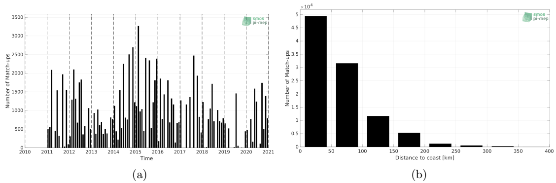
Figure 1: Number of match-ups between TSG (LEGOS-DM) and SMOS SSS L4 OI v342 - Weekly (CMEMS-CATDS-LOPS) SSS as a function of time (a) and as function of the distance to coast (b) over the Mediterranean Sea Pi-MEP region and for the full satellite product period.
