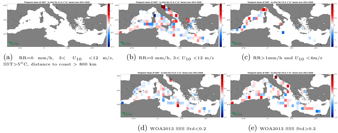
Figure 12: Temporal mean gridded over spatial boxes of size 1^{\circ}\times 1^{\circ} of \Delta\text{SSS} (SMOS SSS L4 OI v342 - Weekly (CMEMS-CATDS-LOPS) - TSG (LEGOS-DM)) for 5 different subdatasets corresponding to:RR=0 mm/h, 3 < U_{10} < 12 m/s, SST >5^{\circ}\text{C} , distance to coast > 800 km (a), RR=0 mm/h, 3 < U_{10} < 12 m/s (b), RR >1 mm/h and U_{10} < 4 m/s (c), WOA2013 SSS Std <0.2 (d), WOA2013 SSS Std >0.2 (e).
