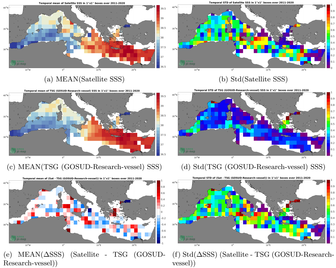
Figure 6: Temporal mean (left) and Std (right) of SSS from SMOS SSS L4 OI v342 - Weekly (CMEMS-CATDS-LOPS) (top), TSG (GOSUD-Research-vessel) ( in situ ) dataset (middle), and of \Delta SSS (Satellite - TSG (GOSUD-Research-vessel)). Only match-up pairs are used to generate these maps.
